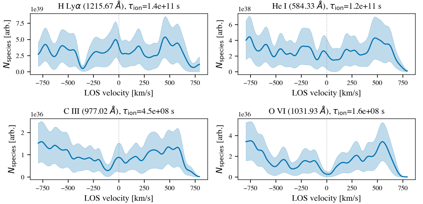
FIG. 7: Predicted Doppler line profiles from the Gaia BH1 wind for four diagnostic UV transitions: H Ly \alpha 1216 Å, He I 584 Å, C III 977 Å, and O VI 1032 Å. Profiles are computed from the line-of-sight velocity histogram of the 1177 steady-state superparticles at i = 126.6^\circ ([1]), binned at \Delta v \approx 13 \text{ km s}^{-1} over [-800, +800] \text{ km s}^{-1} and convolved with a Gaussian thermal width \sigma_{\text{th}} = 30 \text{ km s}^{-1} . Each species is weighted by its X-ray photoionization lifetime \tau_{\text{ion}} [36] under L_X = 10^{29} \text{ erg s}^{-1} [1]. Shaded bands give the per-bin Poisson uncertainty \sqrt{\sum_i w_i^2} . Integration: REBOUND [27], REBOUNDx gr_full [4], MERCURIUS hybrid [30], T_{\text{sim}} = 372 \text{ d} , MC seed = 42.
