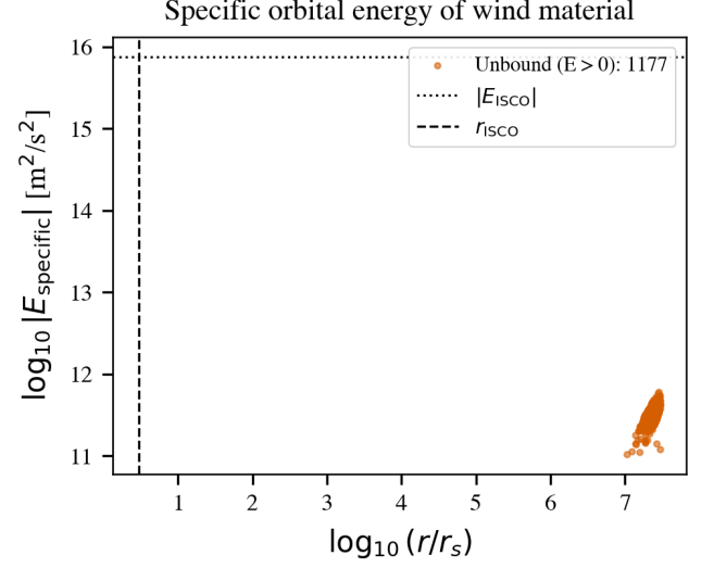
FIG. 9: Specific orbital energy diagram for all 1177 active wind superparticles, plotted as \log_{10} |E| versus \log_{10}(r/r_s) with r_s = 28.4 \text{ km} for the 9.6 M_\odot Gaia BH1 primary. All particles have E > 0 (unbound) and reside at r \gg r_{\text{ISCO}} = 3 r_s (vertical dashed line). No particle crosses the absorbing inner boundary during the T_{\text{sim}} = 372 d integration, validating that the BHL capture rate is set by the geometry of the wind cone rather than by direct strong-field plunge [9]. Integrator: REBOUND [27], REBOUNDx gr_full [4], MERCURIUS hybrid [30], MC seed = 42.
