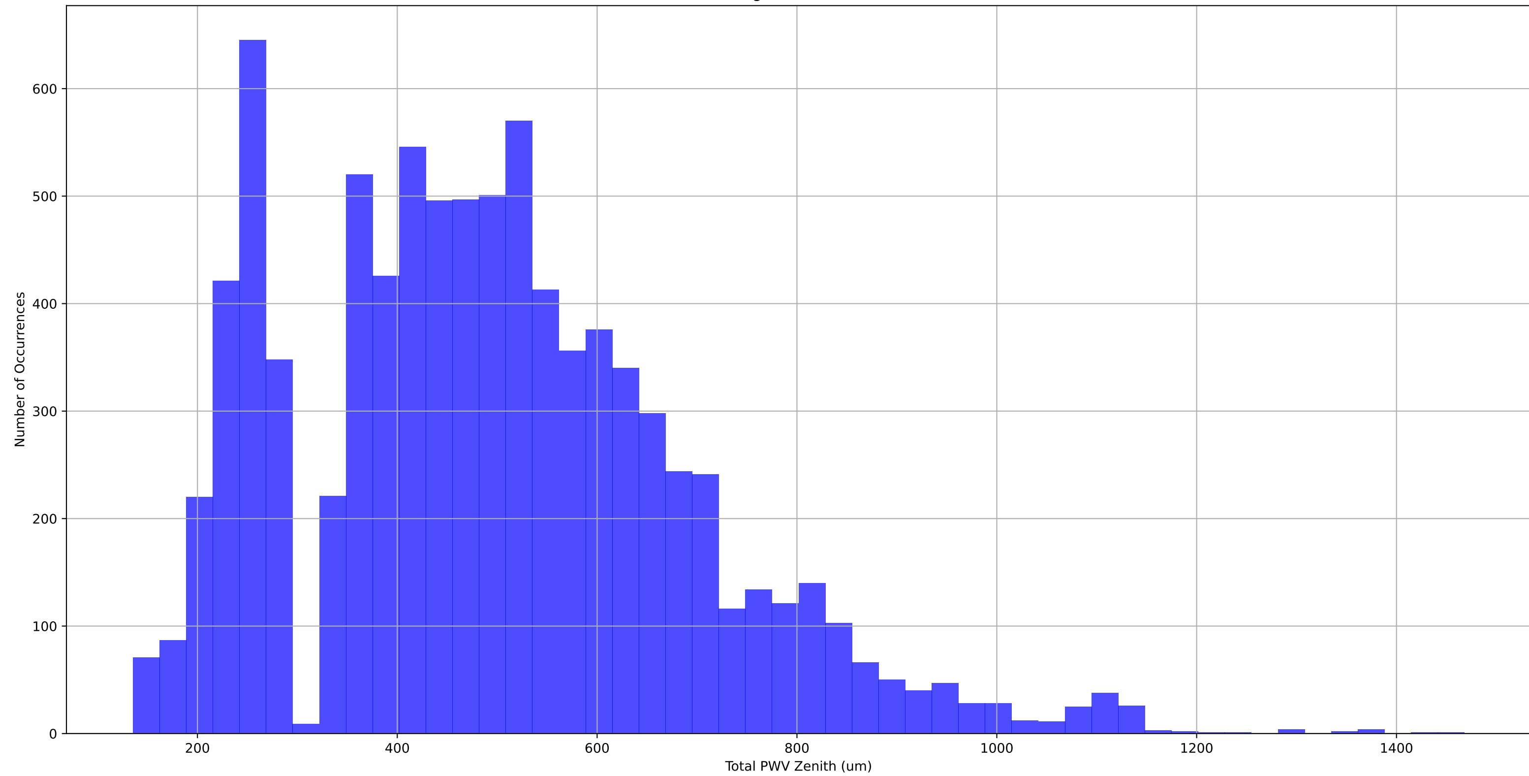
Autumn Histogram of PWV Total Zenith
