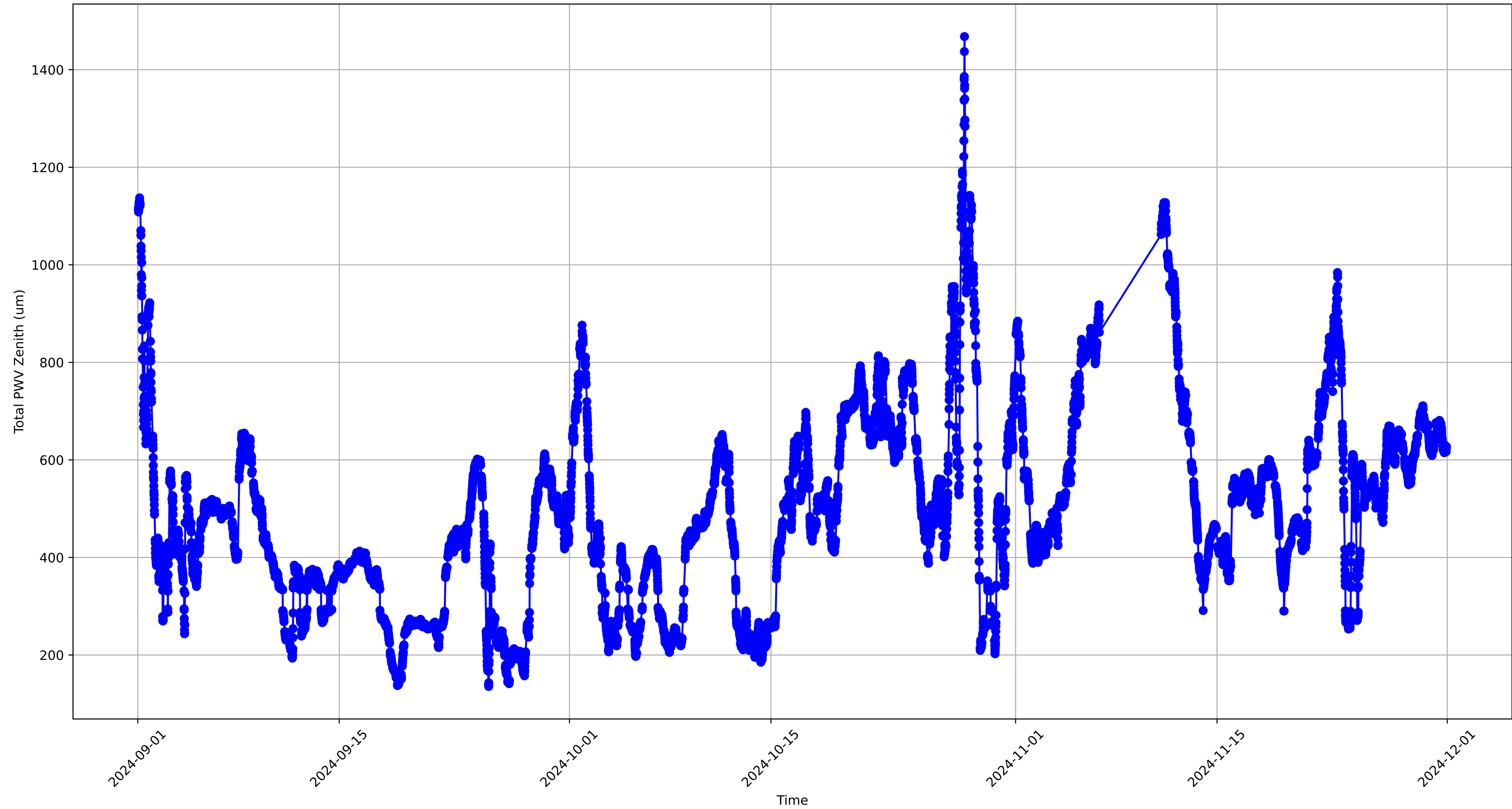
Autumn PWV Total Zenith Over Time
