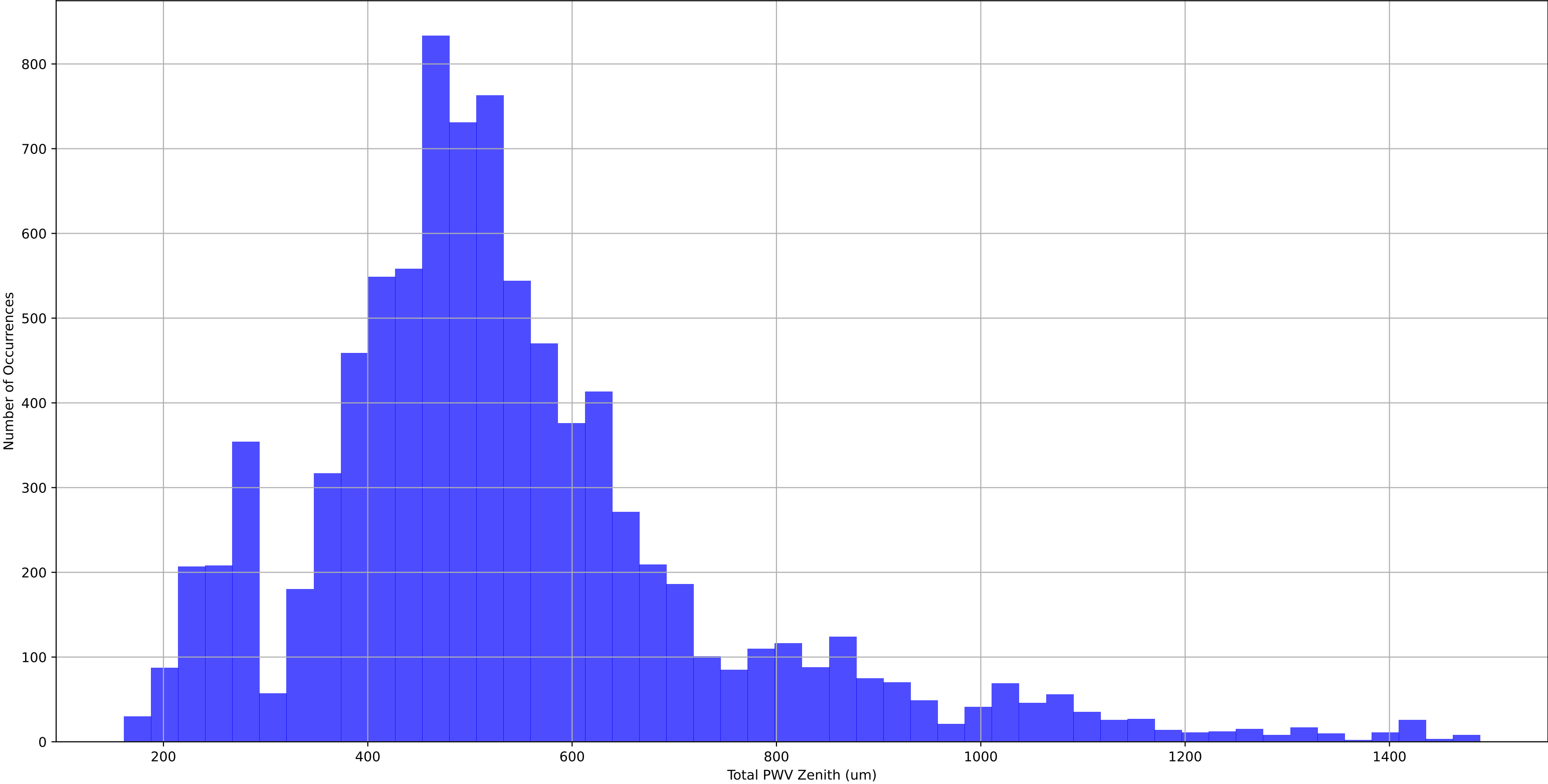
Spring Histogram of PWV Total Zenith
