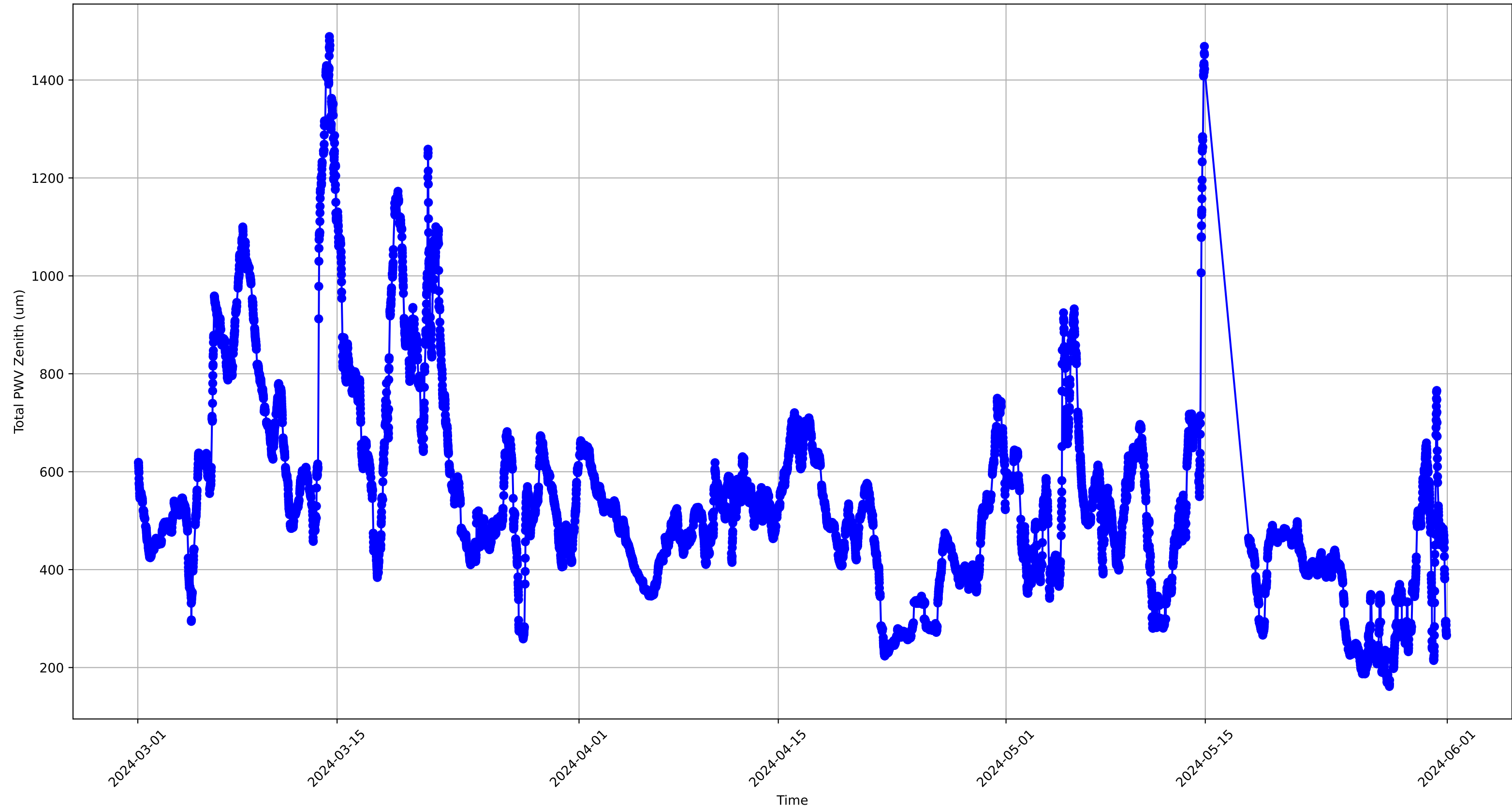
Spring PWV Total Zenith Over Time
