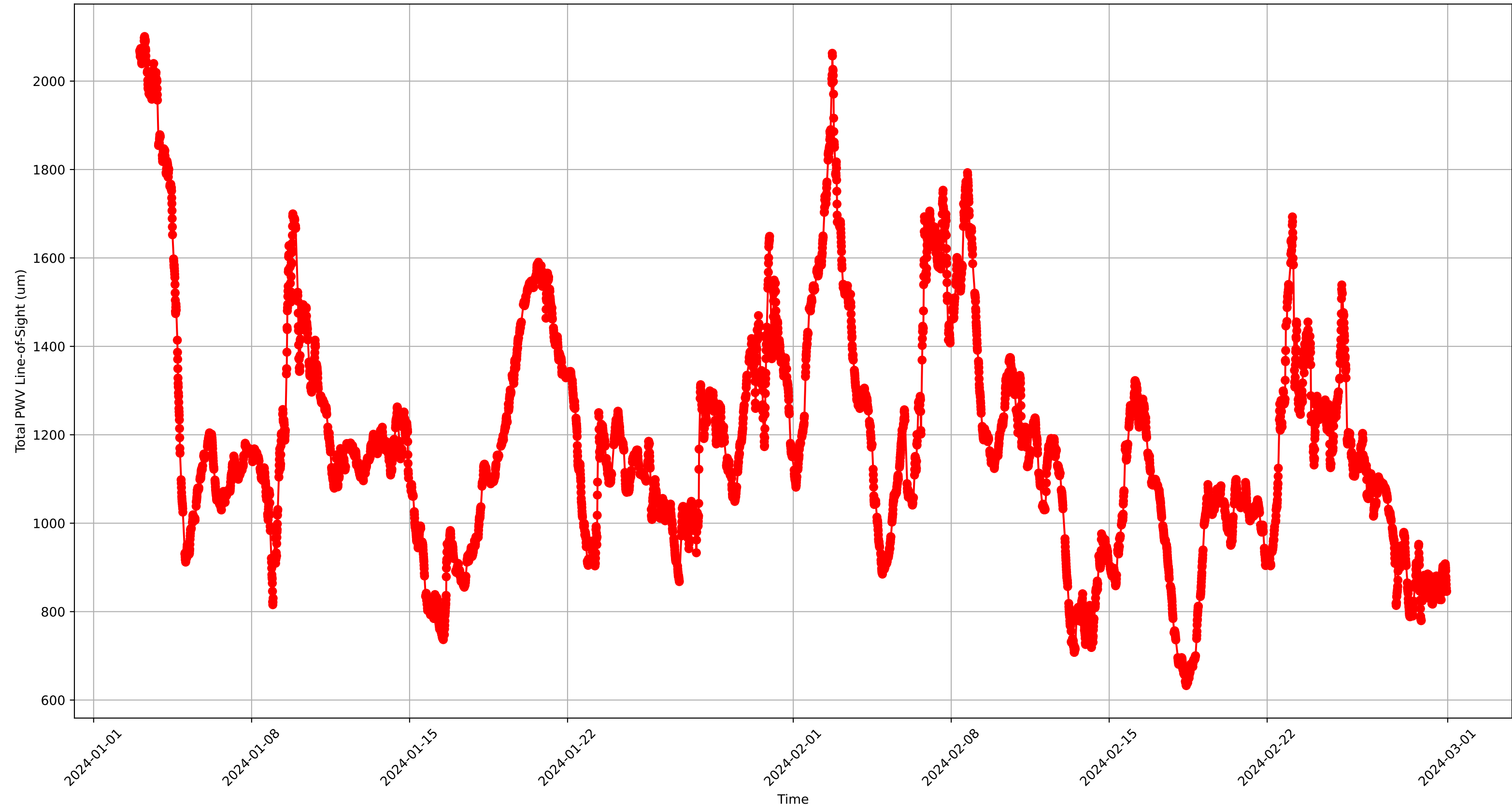
Winter24 PWV Total Line-of-Sight Over Time
