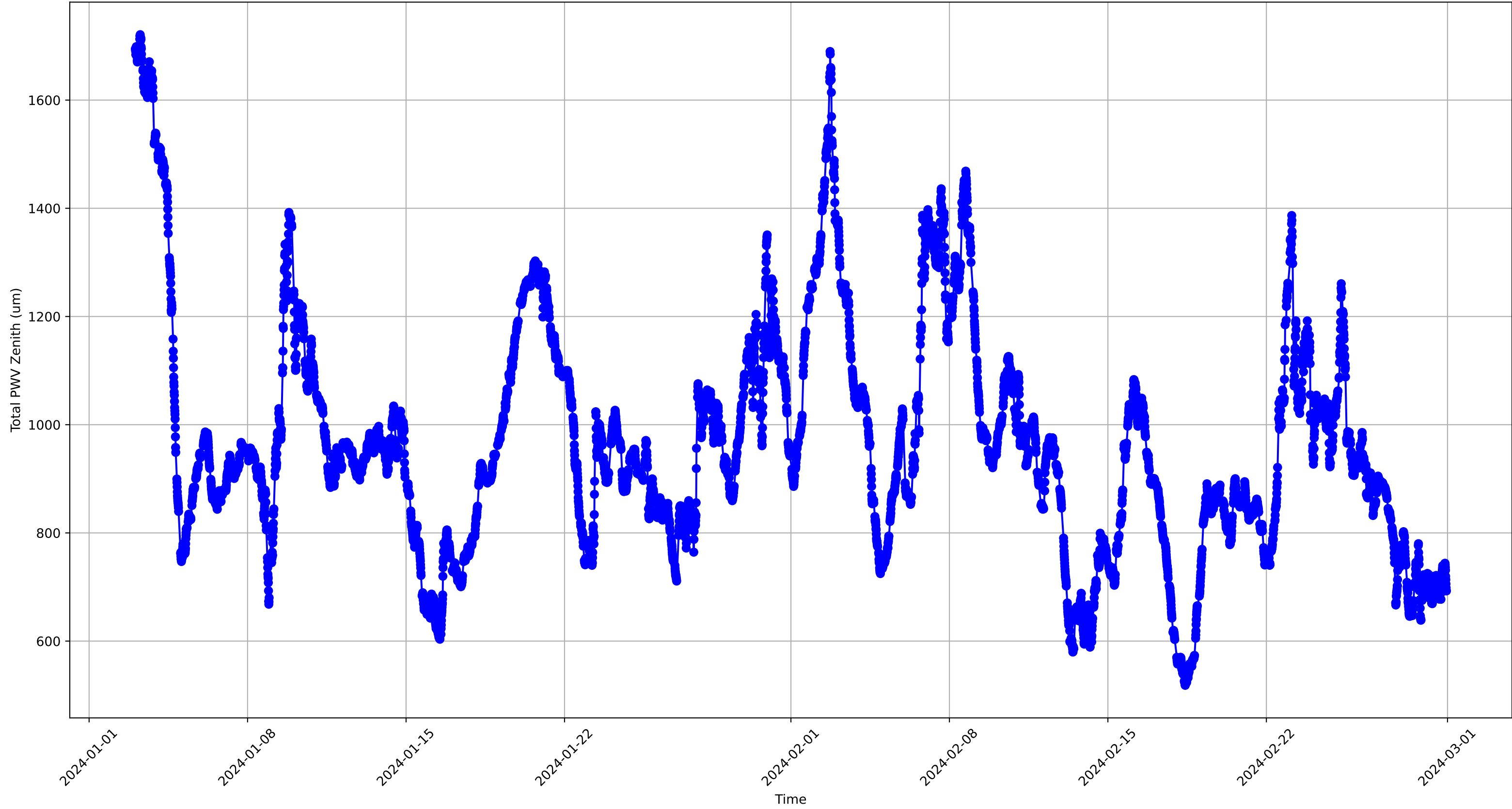
Winter24 PWV Total Zenith Over Time
