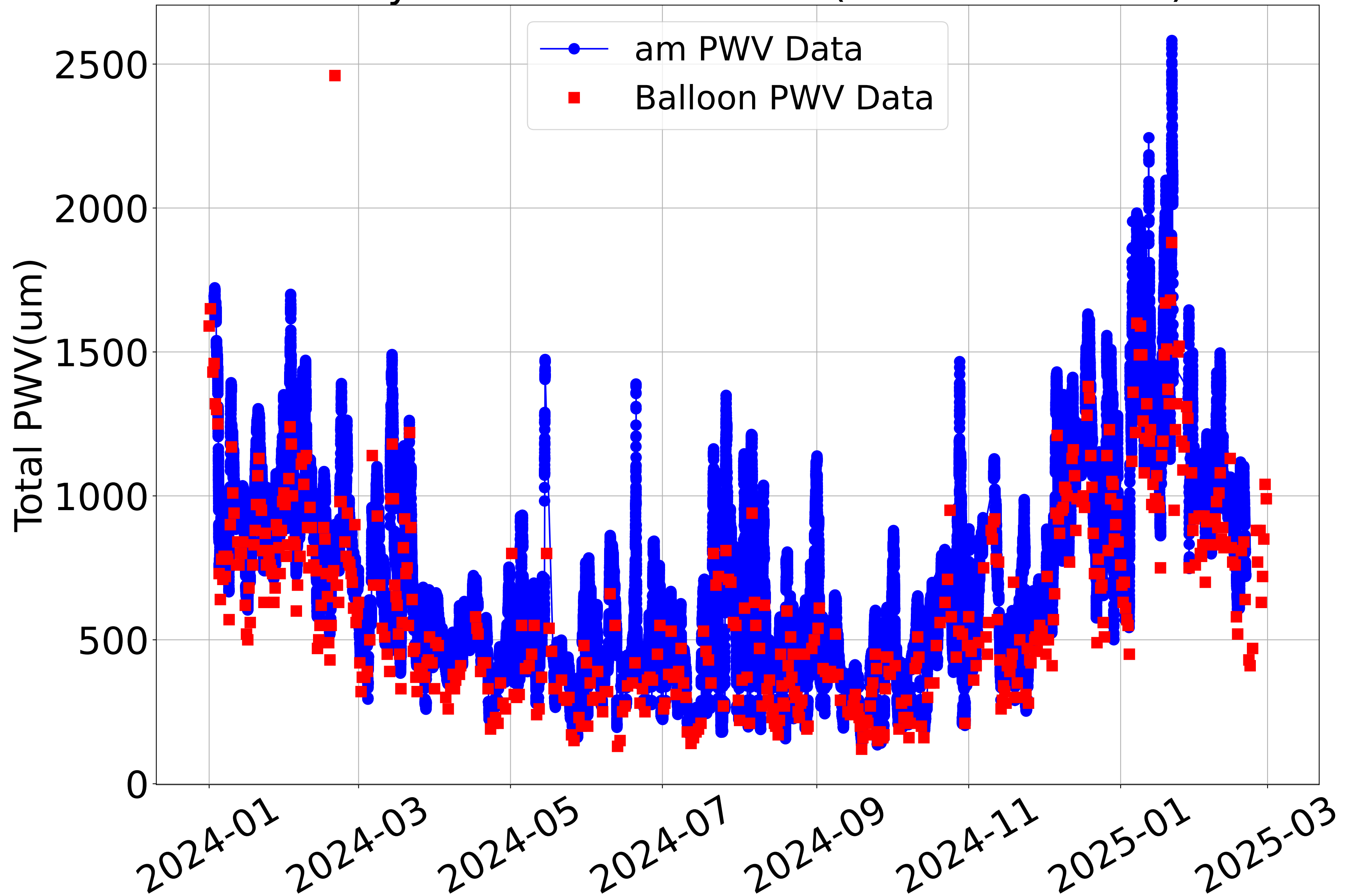
One year PWV Over Time (am and balloon)
