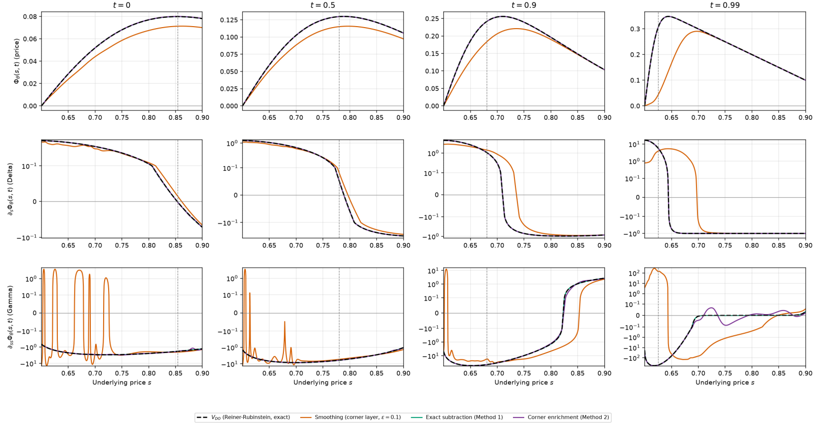
Down-and-out put — price, Delta and Gamma profiles near the corner (one seed) terminal function: Black-Scholes put price (ordinary autograd route); whole domain, corner in collocation
