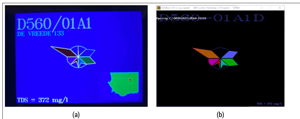
Figure 1. Example of a Maucha diagram from a presentation dated 1989 (a) compared with a diagram generated using the Pascal program in DosBox during 2020 (b).
