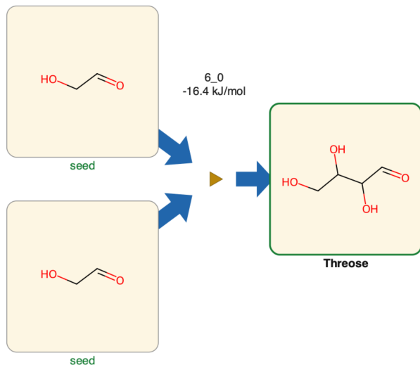
(a) threose, one step
