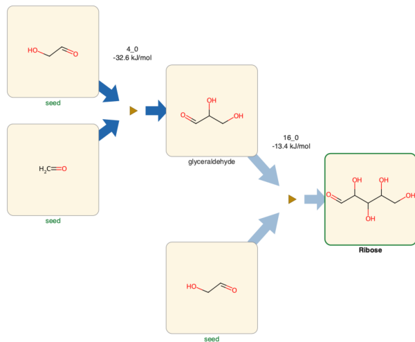
(b) ribose, two steps
