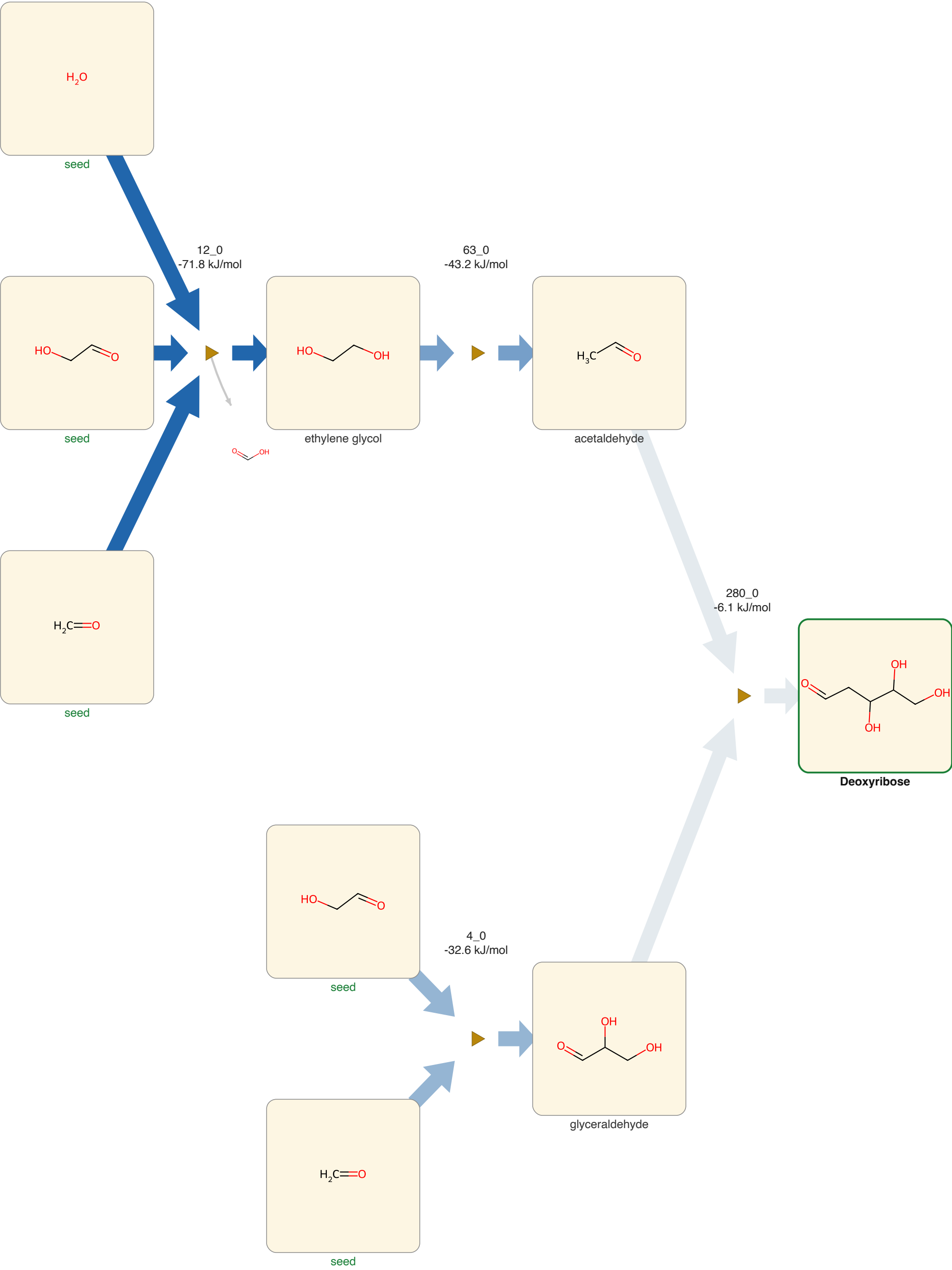
Deoxyribose from Formose, G6, spontaneous reactions, admitting those of unestimable free energy. Structures are constitutional; the network carries no stereochemistry.
