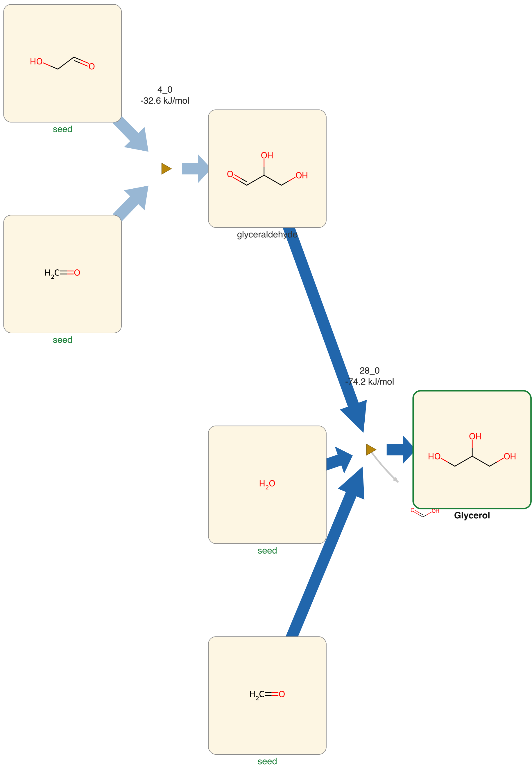
Glycerol from Formose, G6, spontaneous reactions, admitting those of unestimable free energy. Structures are constitutional; the network carries no stereochemistry.
