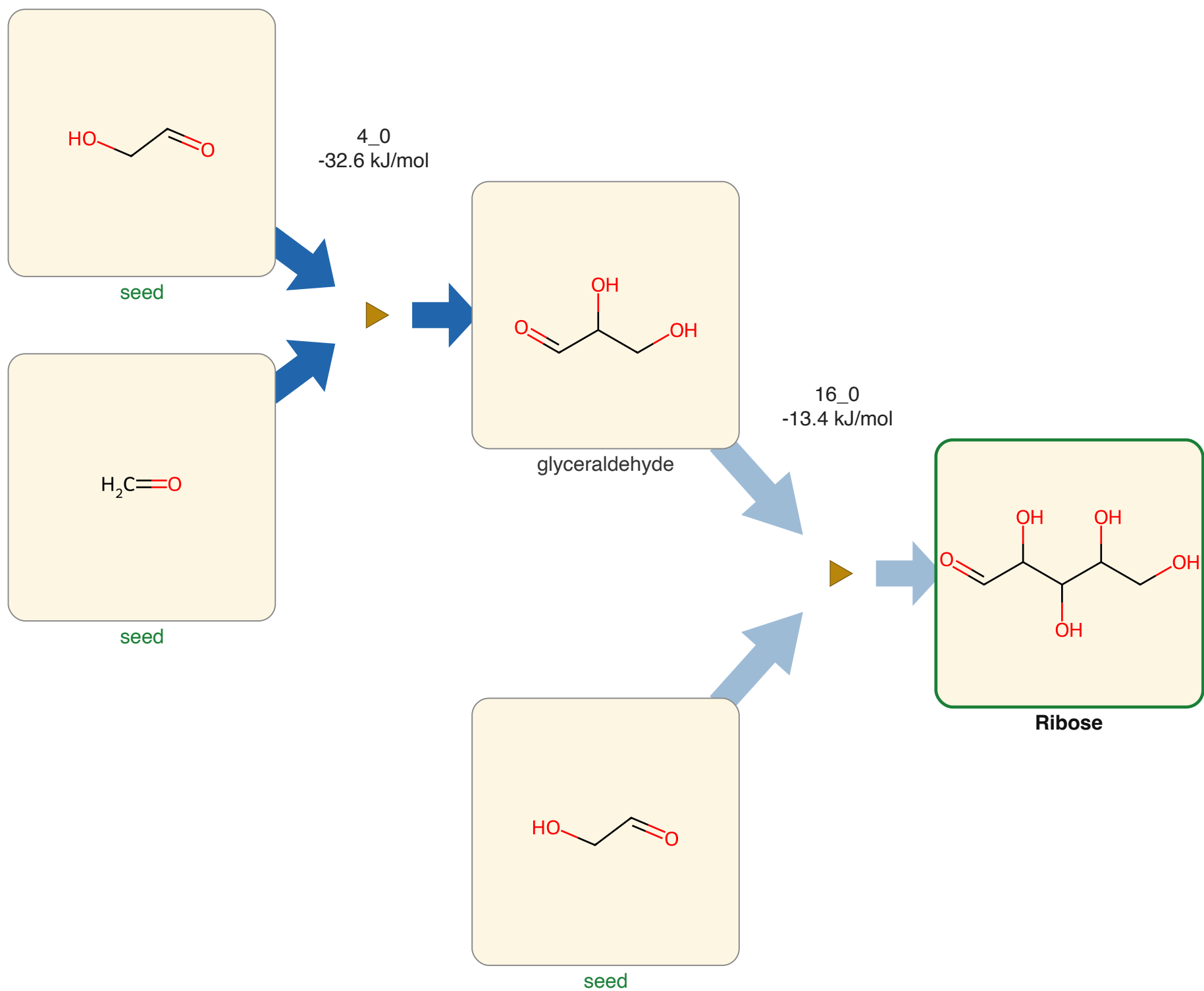
Ribose from Formose, G6, spontaneous reactions, admitting those of unestimable free energy. Structures are constitutional; the network carries no stereochemistry.
