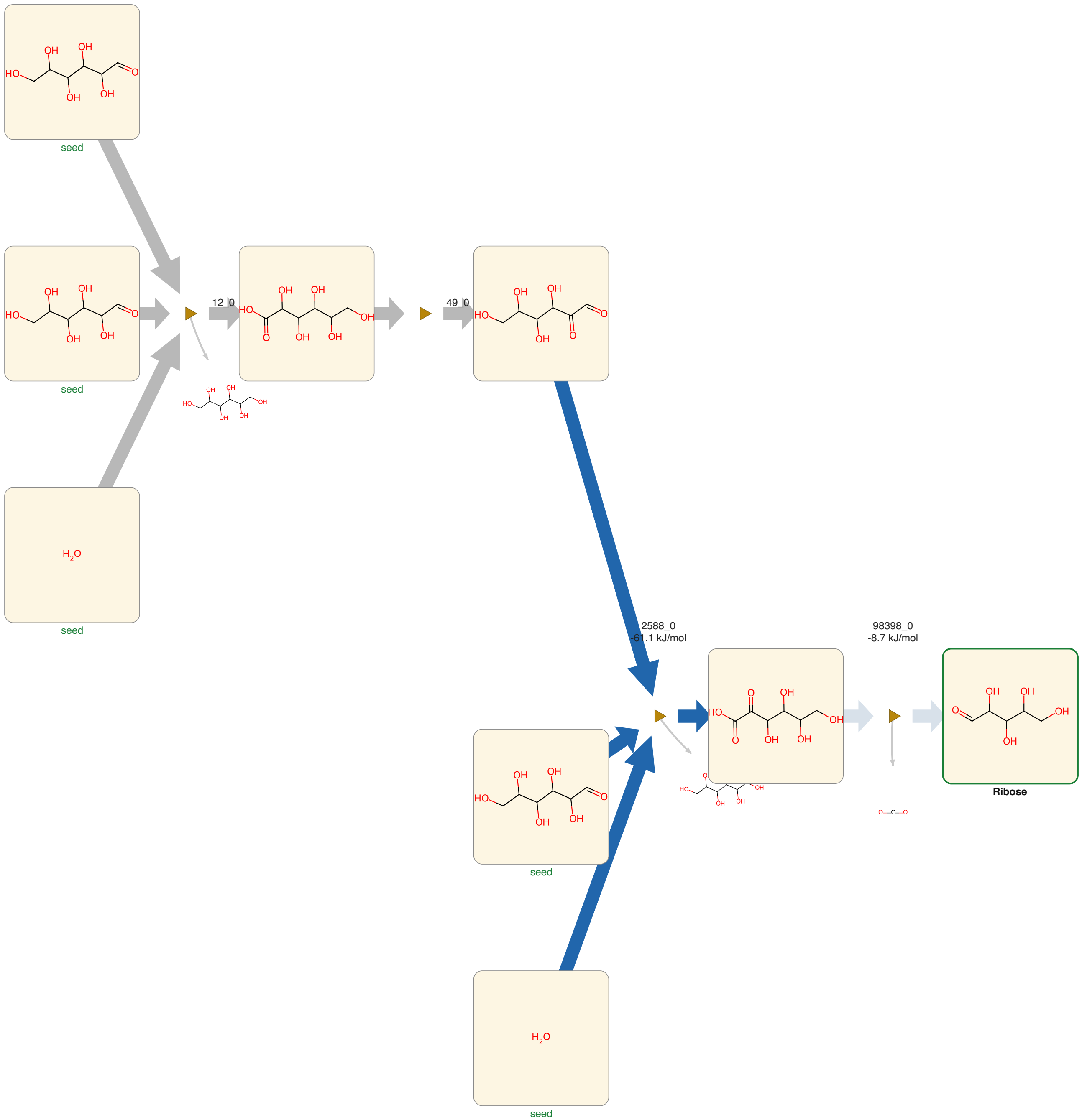
Ribose from GlucoseAmm, G4, spontaneous reactions, admitting those of unestimable free energy. Structures are constitutional; the network carries no stereochemistry.
