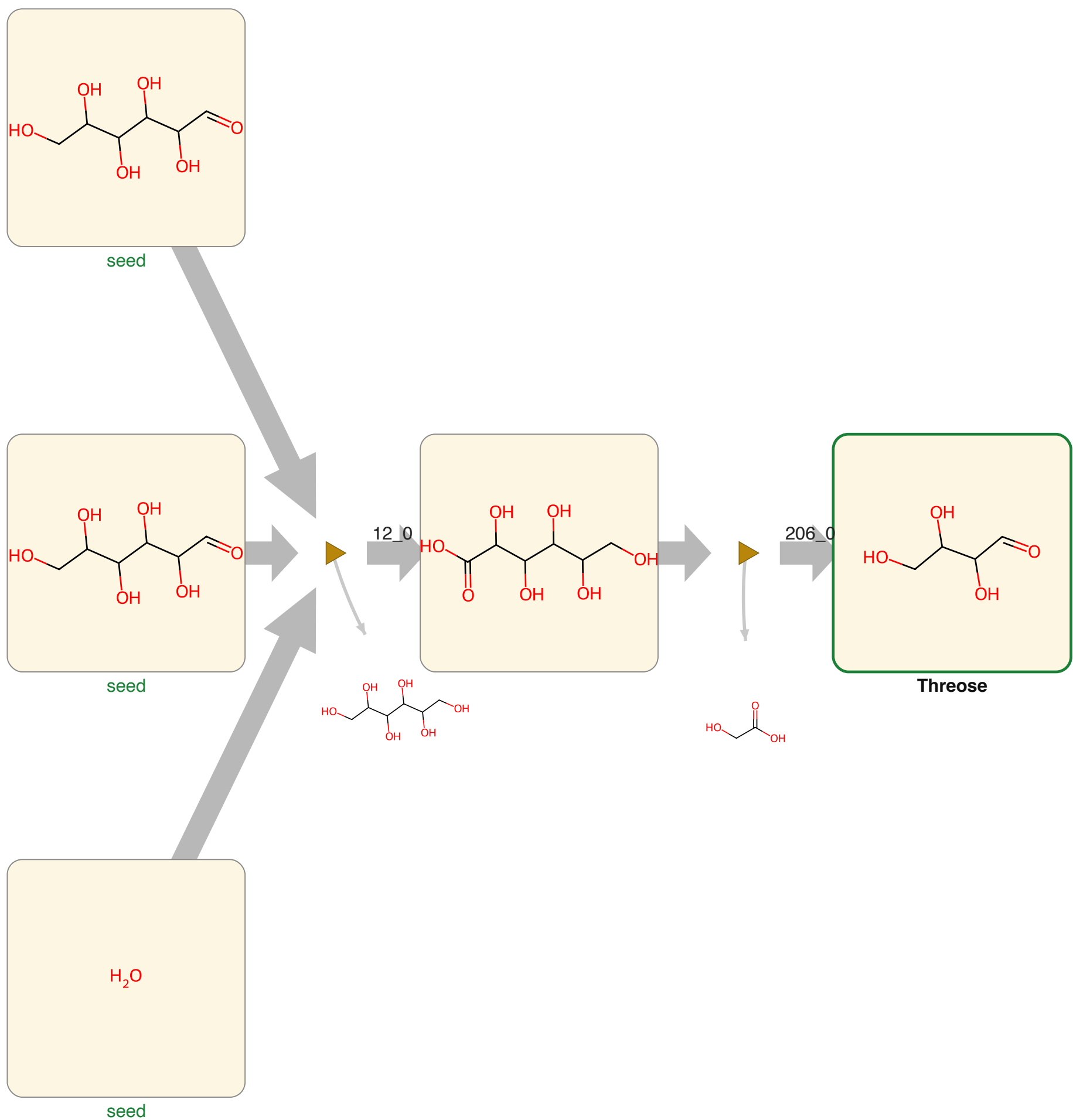
Threose from GlucoseAmm, G4, spontaneous reactions, admitting those of unestimable free energy. Structures are constitutional; the network carries no stereochemistry.
