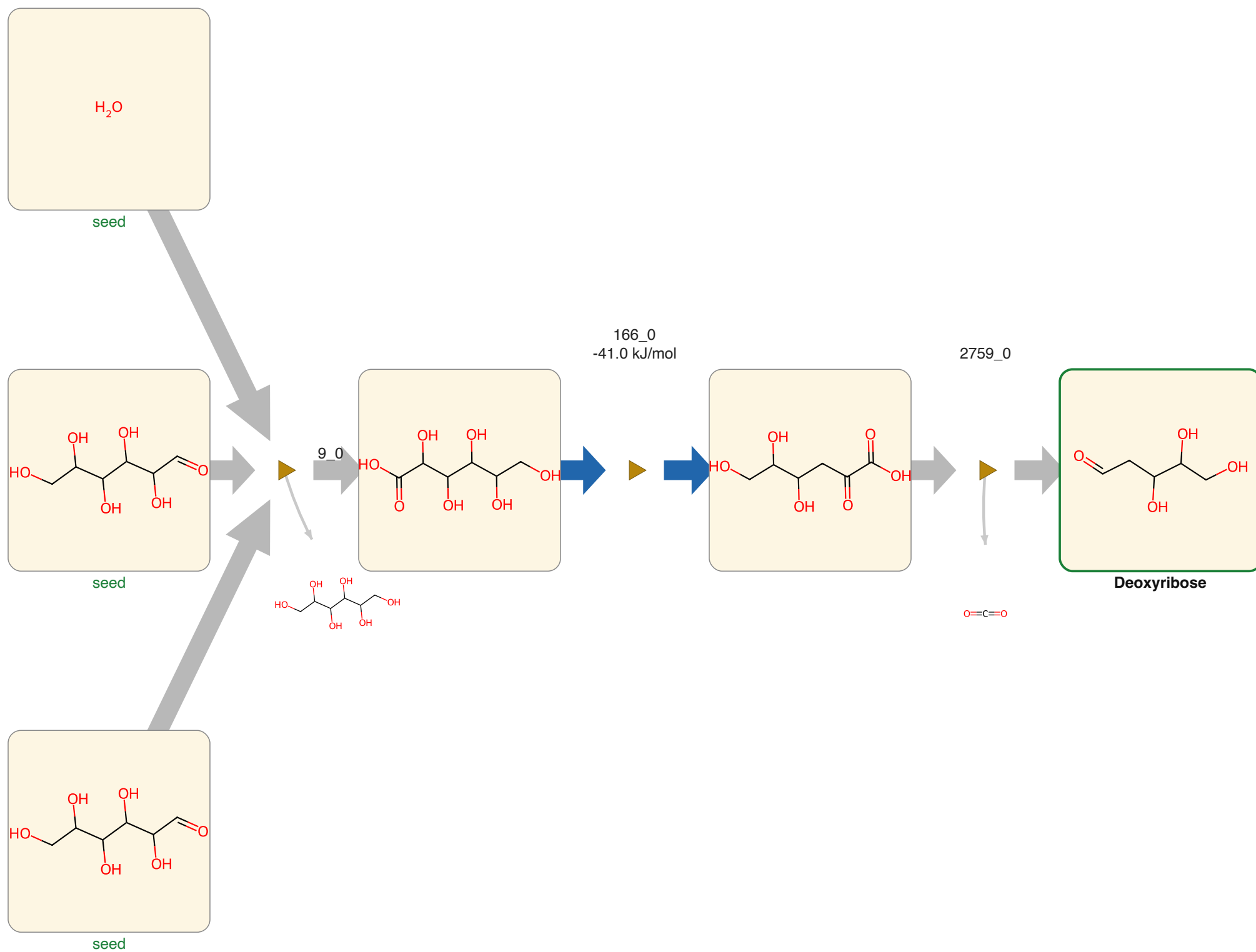
Deoxyribose from Glucose, G5, spontaneous reactions, admitting those of unestimable free energy. Structures are constitutional; the network carries no stereochemistry.
