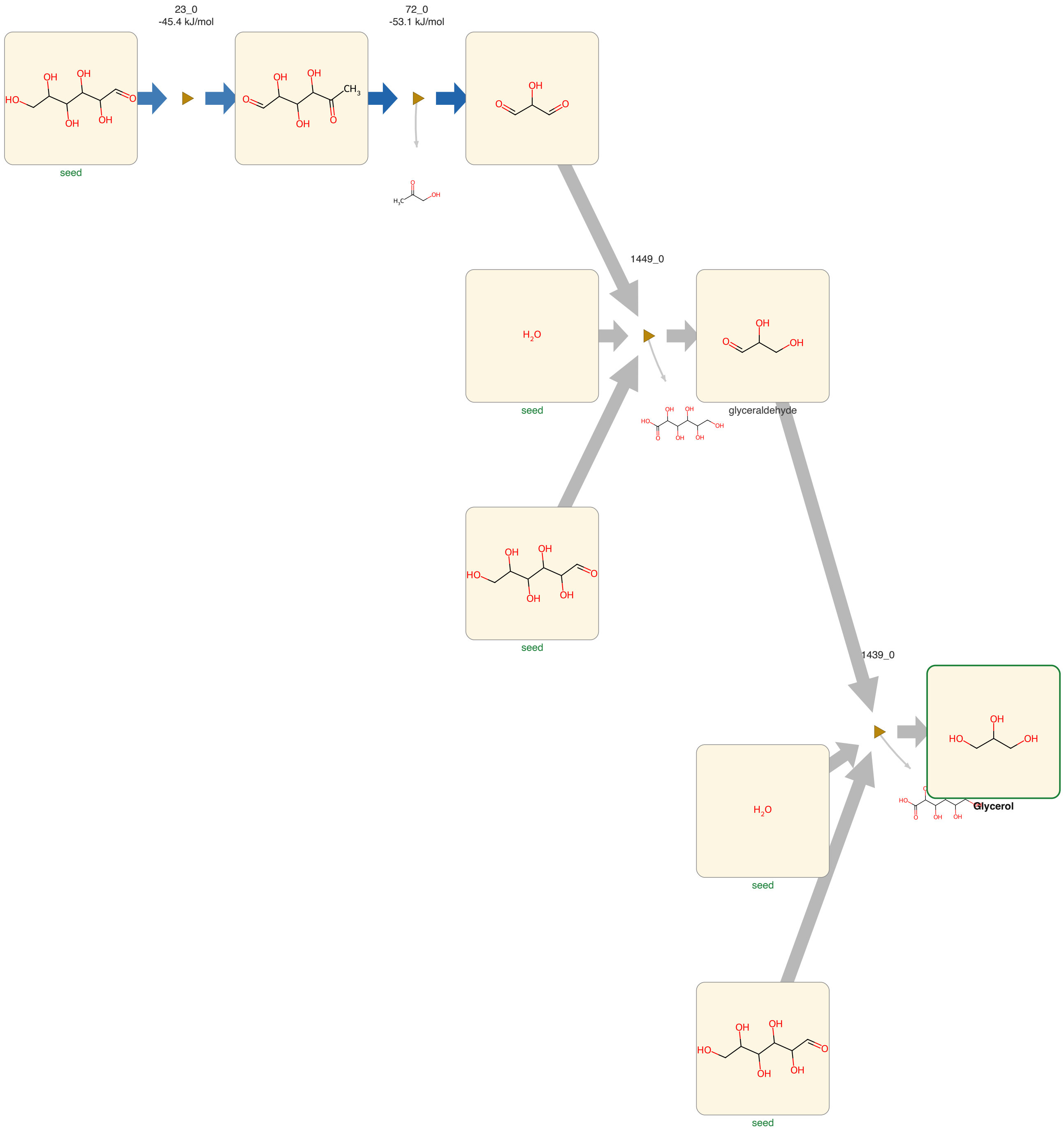
Glycerol from Glucose, G5, spontaneous reactions, admitting those of unestimable free energy. Structures are constitutional; the network carries no stereochemistry.
