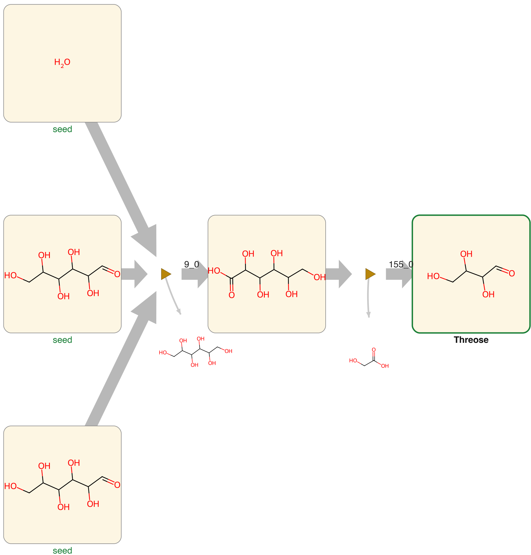
Threose from Glucose, G5, spontaneous reactions, admitting those of unestimable free energy. Structures are constitutional; the network carries no stereochemistry.
