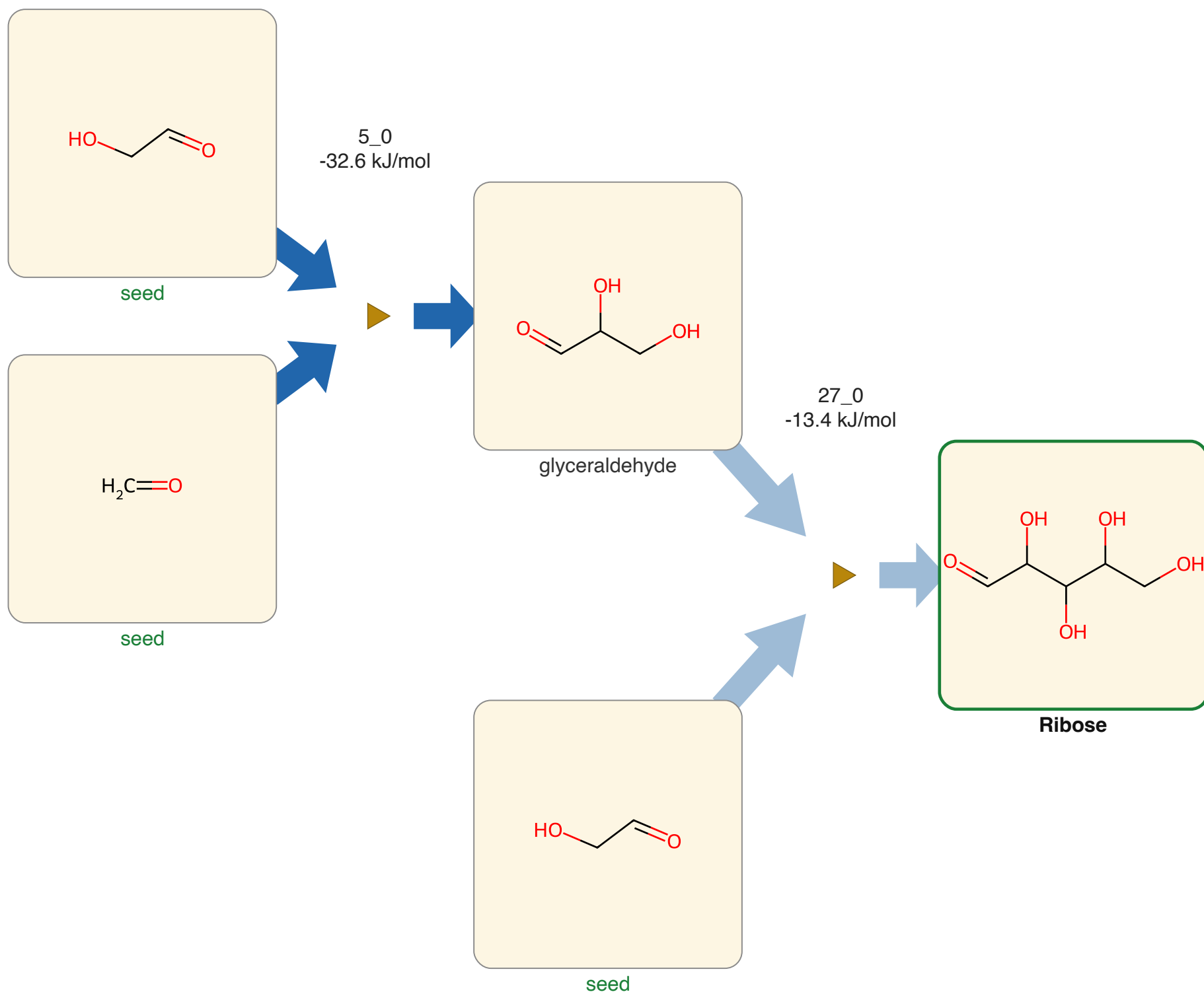
Ribose from FormoseAmm, G4, spontaneous reactions only. Structures are constitutional; the network carries no stereochemistry.
