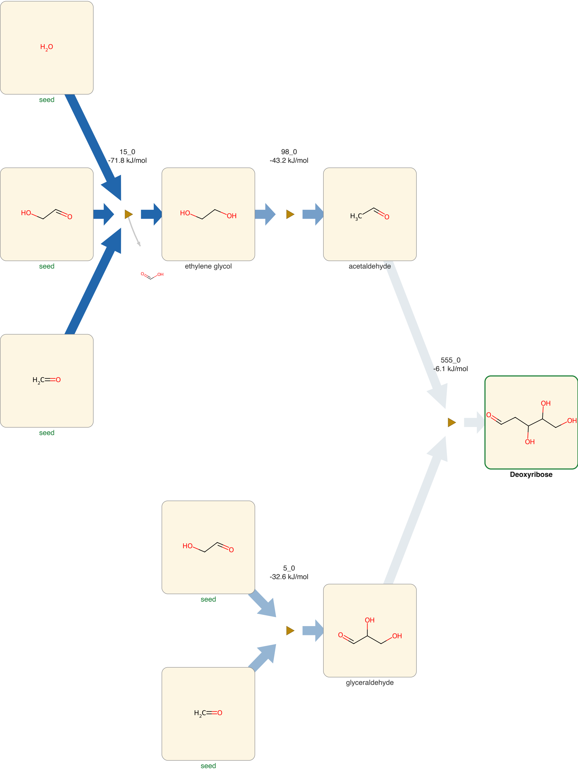
Deoxyribose from FormoseAmm, G4, spontaneous reactions only. Structures are constitutional; the network carries no stereochemistry.
