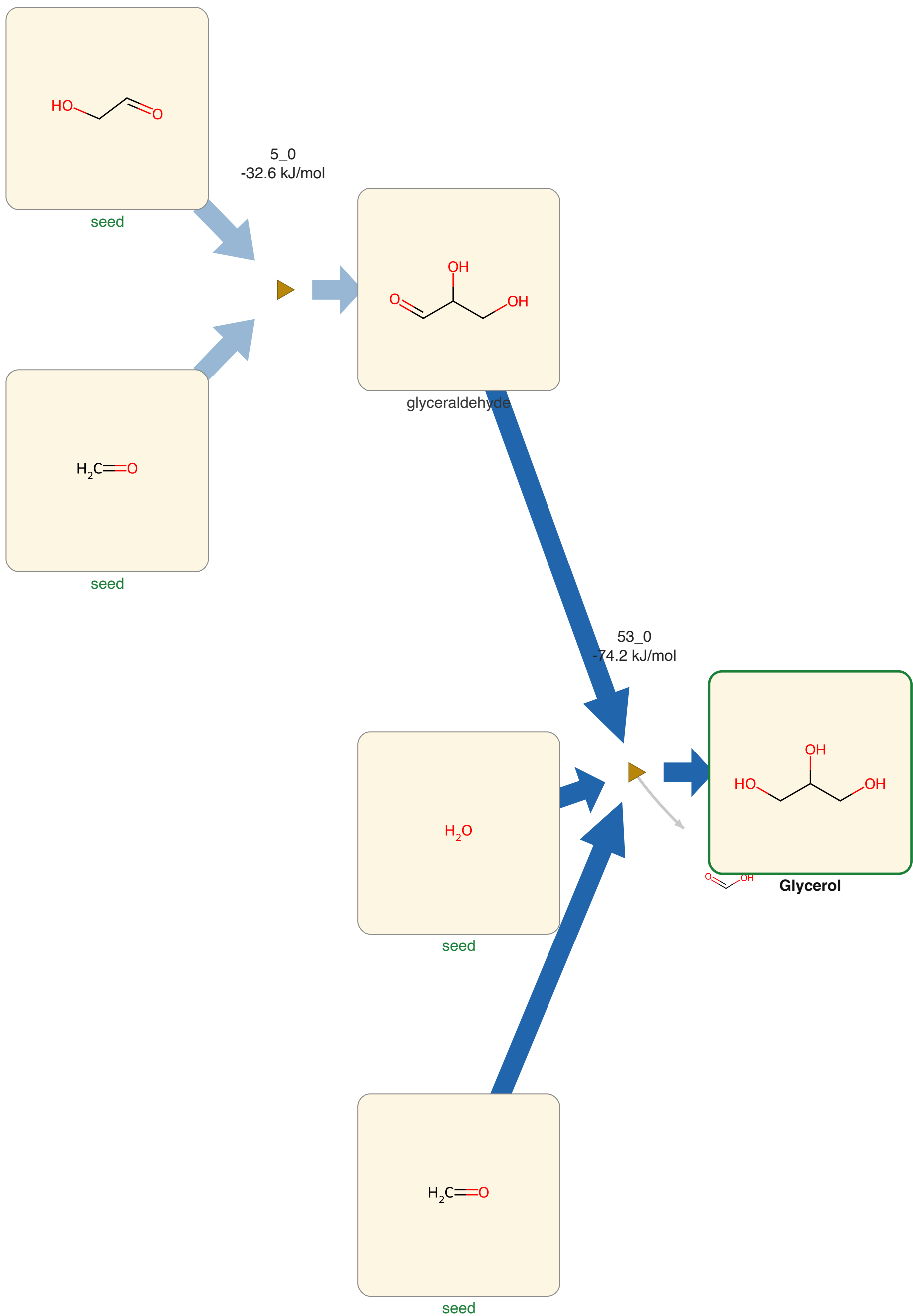
Glycerol from FormoseAmm, G4, spontaneous reactions only. Structures are constitutional; the network carries no stereochemistry.
