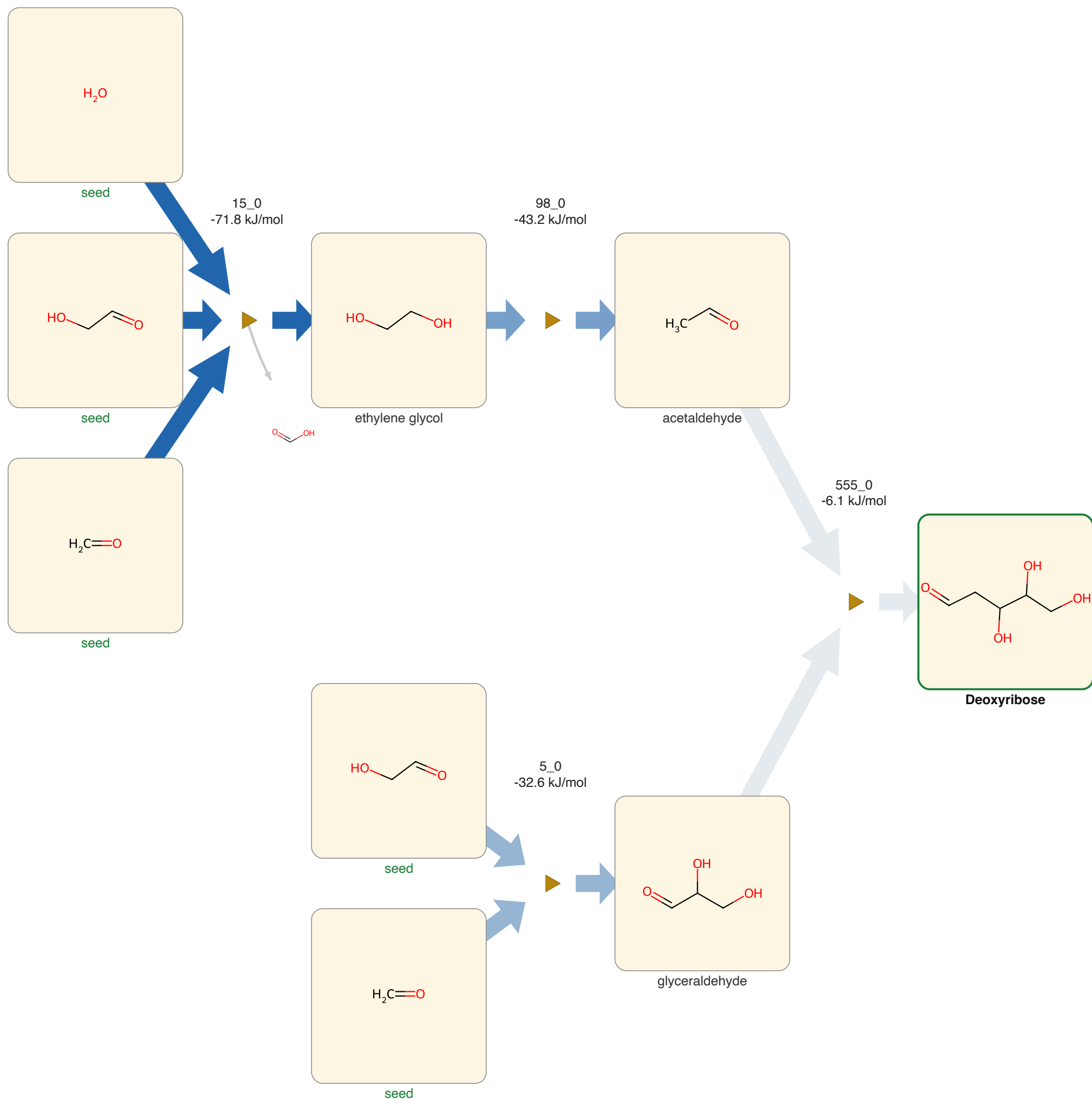
Deoxyribose from FormoseAmm, G4, spontaneous reactions only. Structures are constitutional; the network carries no stereochemistry.
