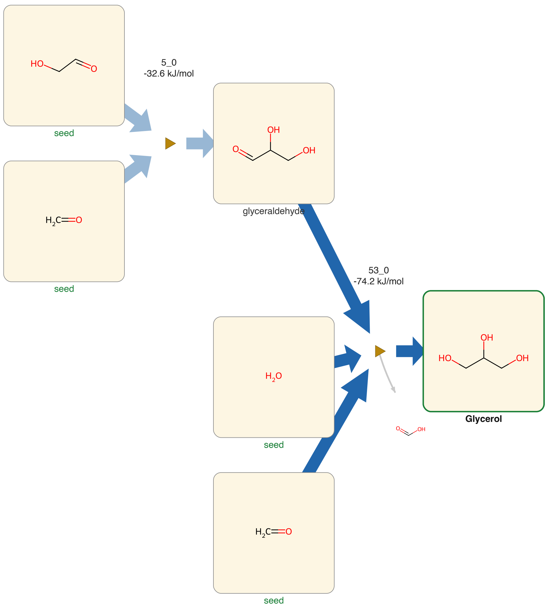
Glycerol from FormoseAmm, G4, spontaneous reactions only. Structures are constitutional; the network carries no stereochemistry.
