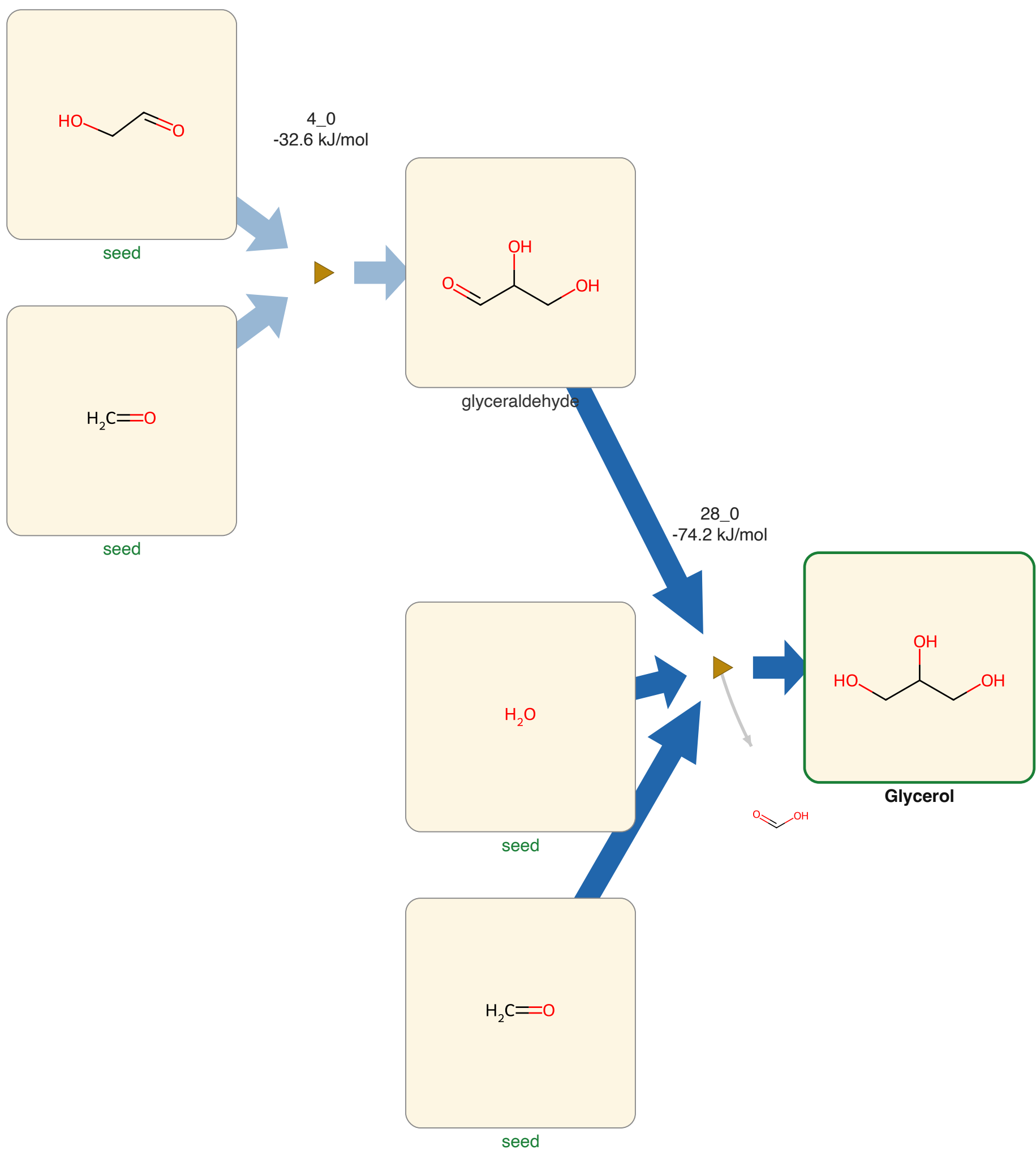
Glycerol from Formose, G6, spontaneous reactions only. Structures are constitutional; the network carries no stereochemistry.
