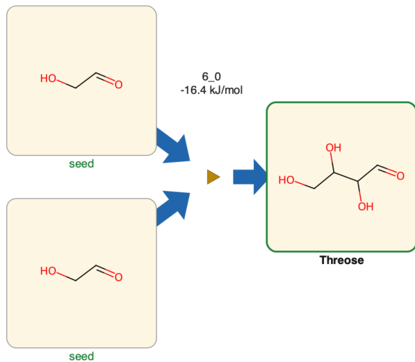
(a) threose, one step
