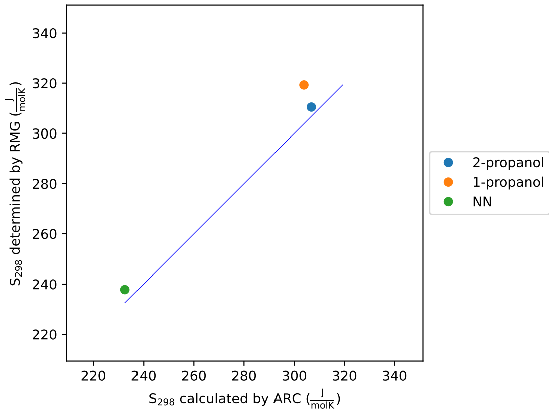
S_{298} parity plot
