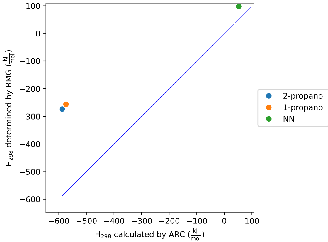
H 298 parity plot
