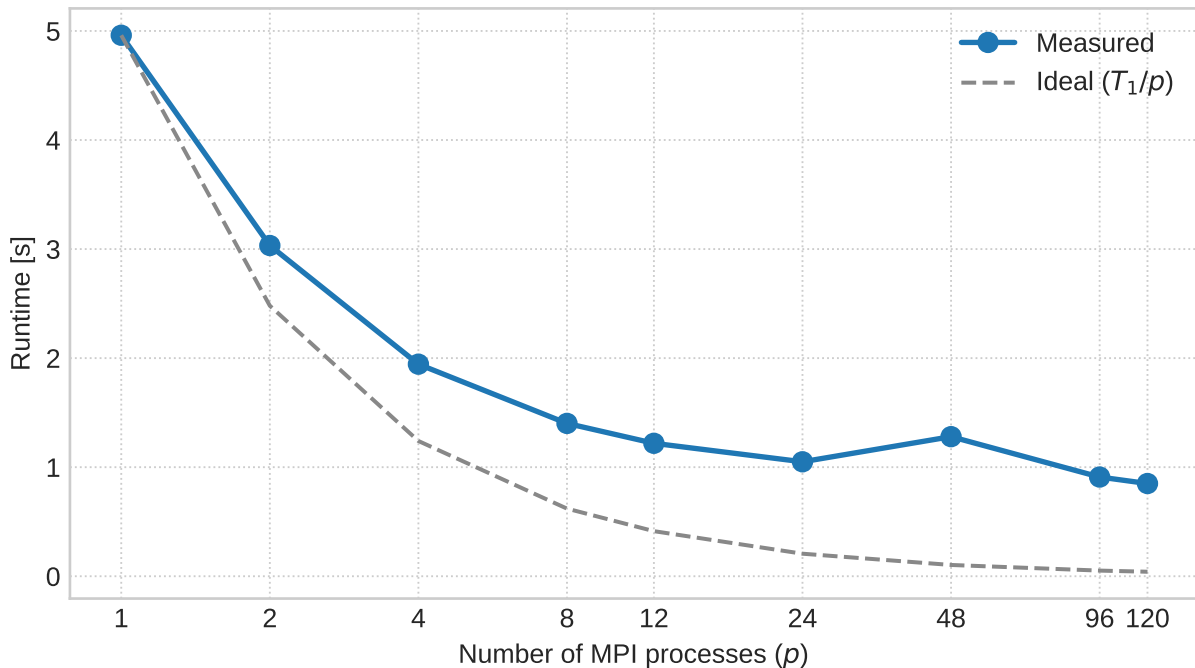
Strong scaling — Janna/Hook_1498 (Okeanos)
