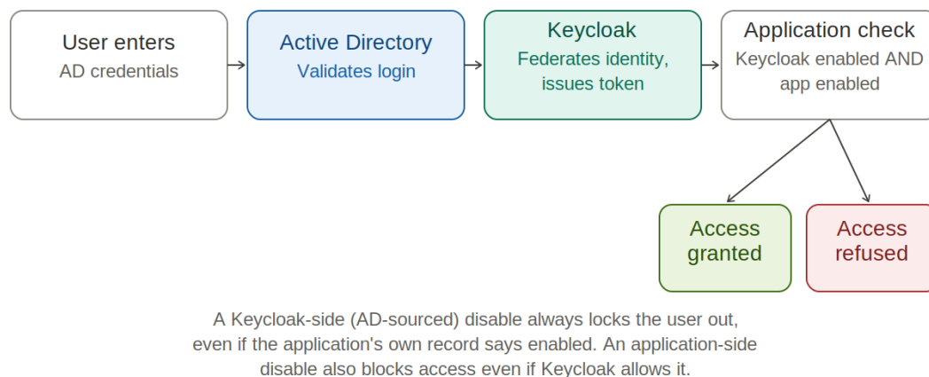
Figure 5.2: Account status after AD federation. Access requires two conditions to hold at once, checked on every request: the account must be enabled in Keycloak, whose status is itself now sourced from AD through federation, and enabled in the application's own record.
