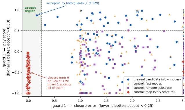
Figure 3: Both L2 guards on 129 chaotic systems from Gilpin [2021]; one marker per (system, candidate reduction). The red stripe at closure error 0 is the reduction that maps every state to zero: it satisfies guard 1 on 124 of 129 systems and is held out of the accept region only by the pay axis, never rising above -0.030 . Closure errors that were non-finite or exceeded 3 are parked at the right edge.
