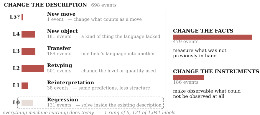
Figure 2: What a discovering system has to be able to do. A move changes the facts you hold, the instruments you have, or the description you use; only a change of description has a depth, and its six rungs are regression (L0), solving inside the description you already have; reinterpretation (L1), the same predictions with less structure; retyping (L2), changing the level or quantity it is written in; transfer (L3), carrying another field's language in; new object (L4), adding a kind of thing the language lacked; and new move (L5), changing what counts as a move. The three column totals are annotated prize events across all fields; the per-rung counts are depth labels, since an event may sit on more than one rung (1,041 labels across 1,547 events). Of the fourteen systems we surveyed, all predominantly operate within a predefined representational or operator language; L5 is a single event its annotator flagged uncertain.
