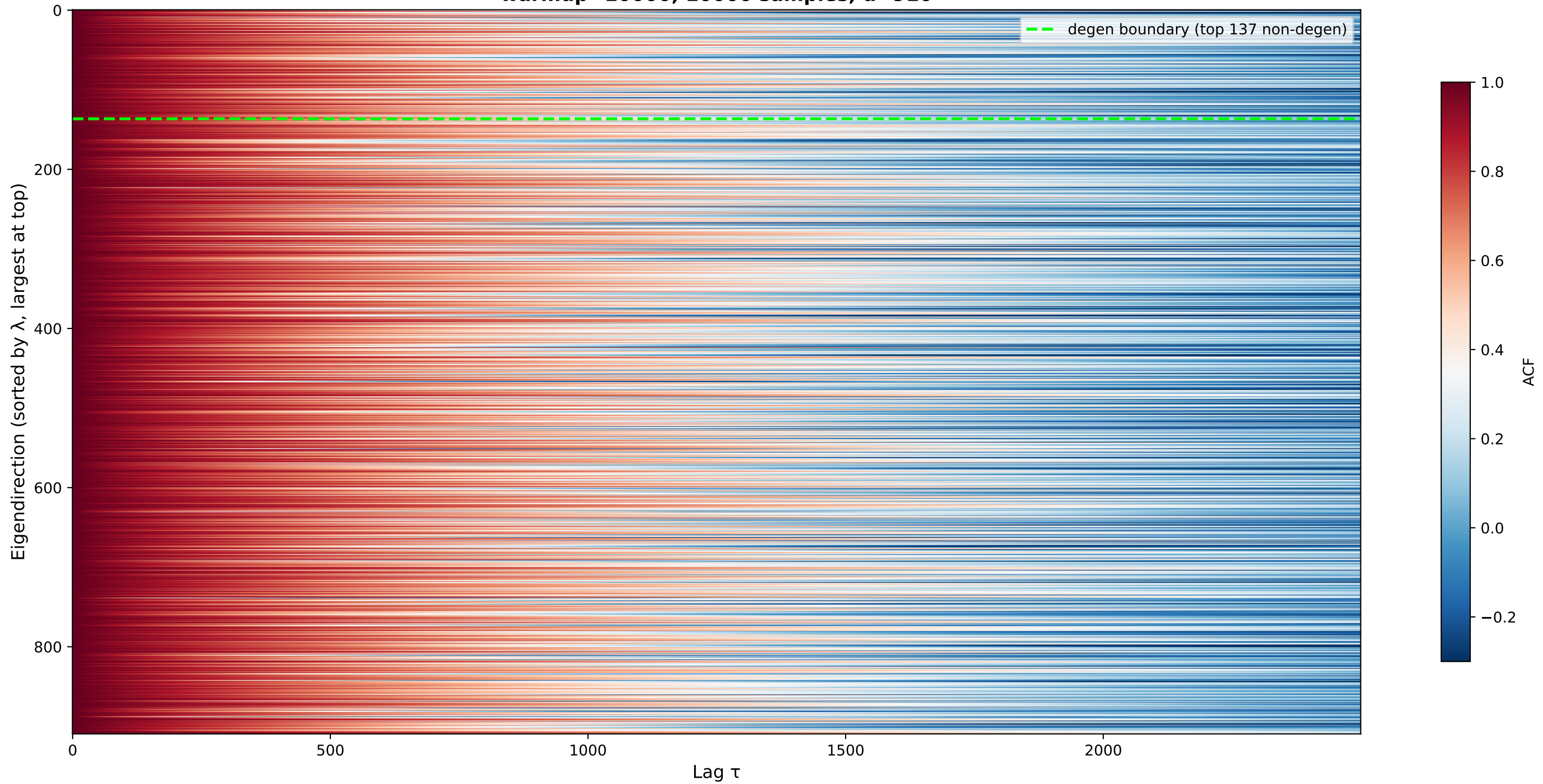
ACF per Hessian eigendirection — NUTS, identity M + adaptation warmup=10000, 10000 samples, d=910
