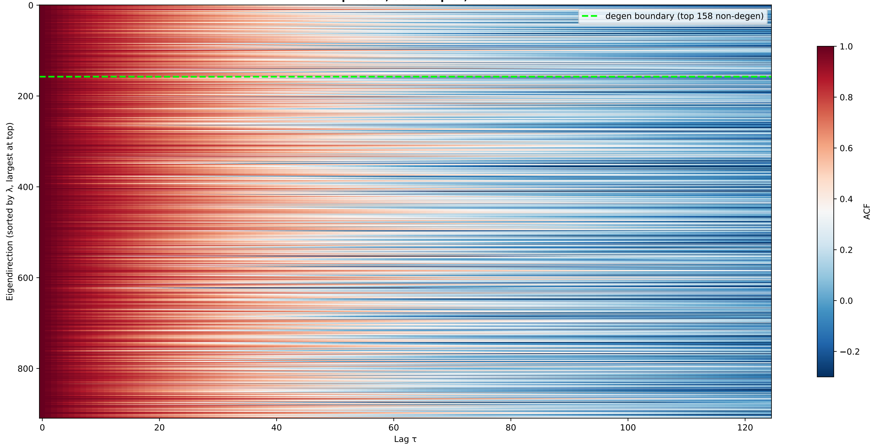
ACF per Hessian eigendirection — NUTS, identity M + adaptation warmup=2000, 500 samples, d=910
