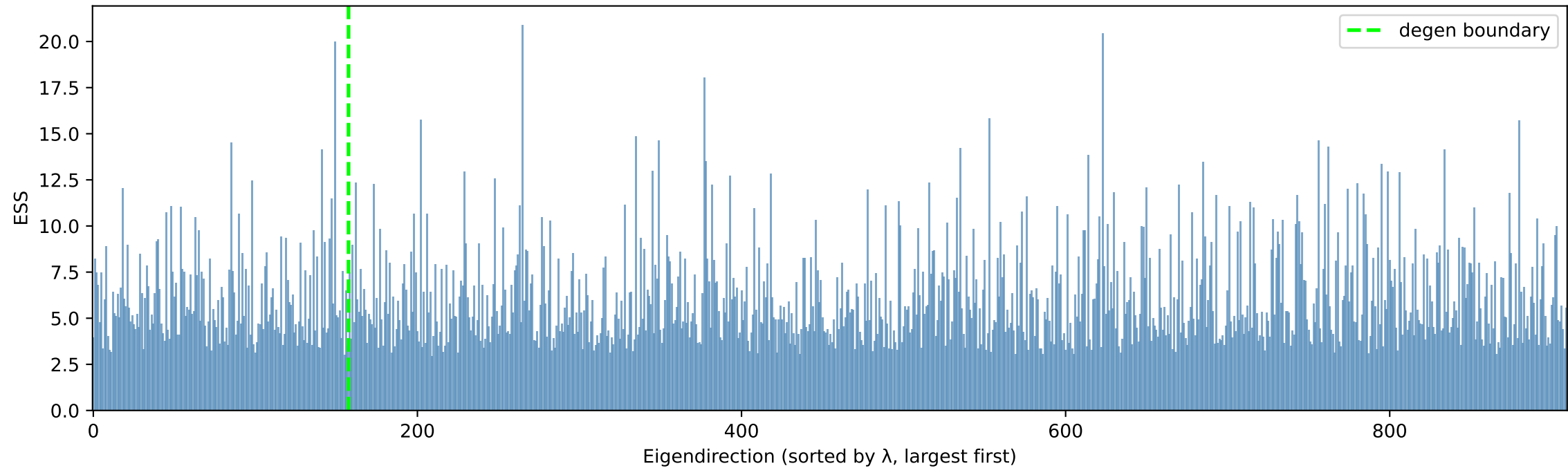
Effective Sample Size per eigendirection (N=500)
