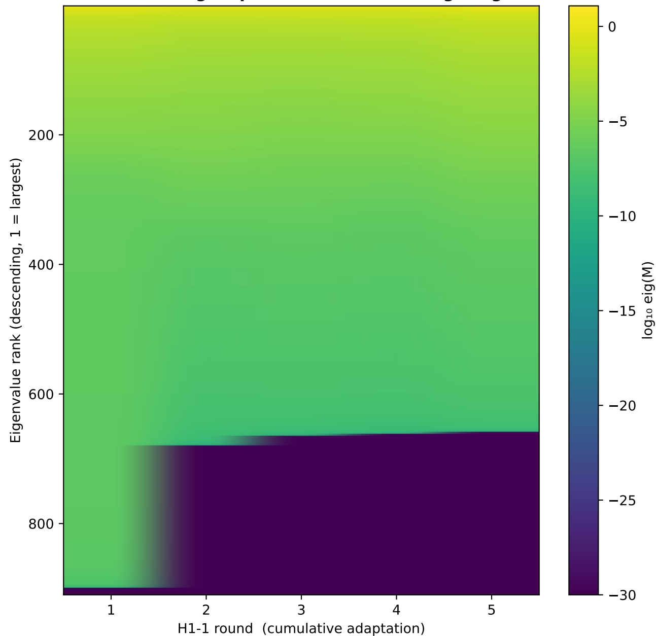
Mass matrix eigenspectrum evolution ( \log_{10} \text{eig}(M) )
