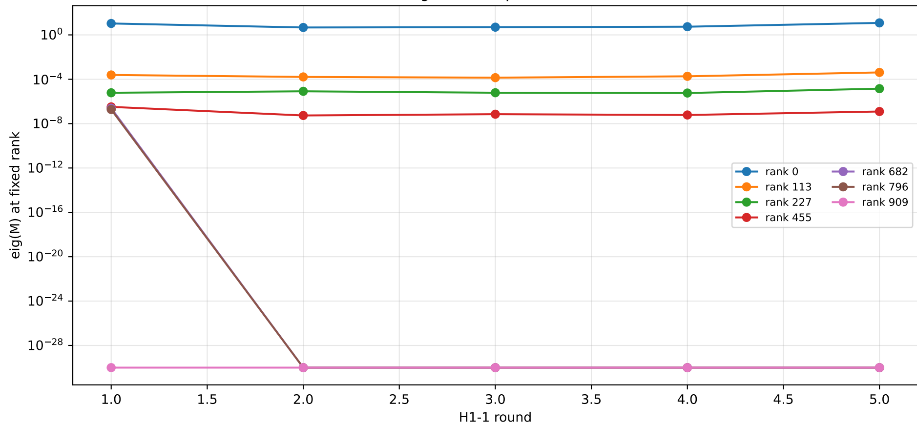
Mass matrix eigenvalues per rank across rounds
