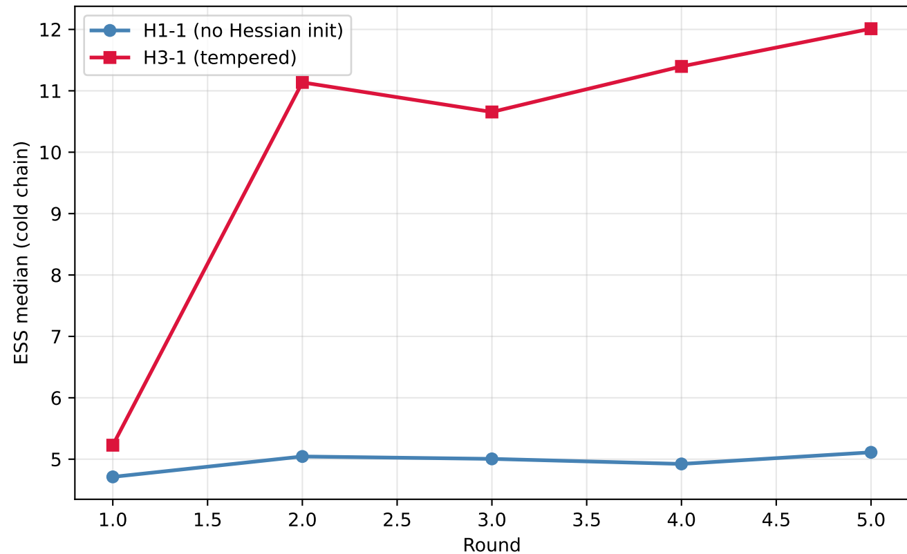
ESS: H3-1 vs H1-1
