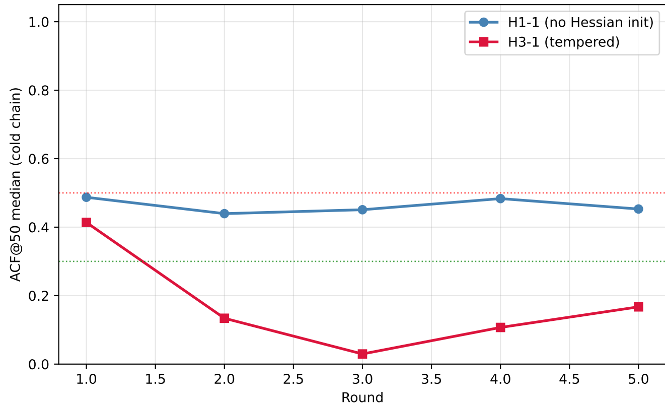
ACF@50: H3-1 vs H1-1
