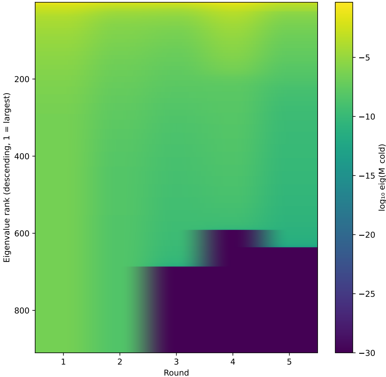
Cold-chain mass matrix eigenspectrum evolution ( \log_{10} \text{ eig}(\mathbf{M}_{\text{cold}}) )
