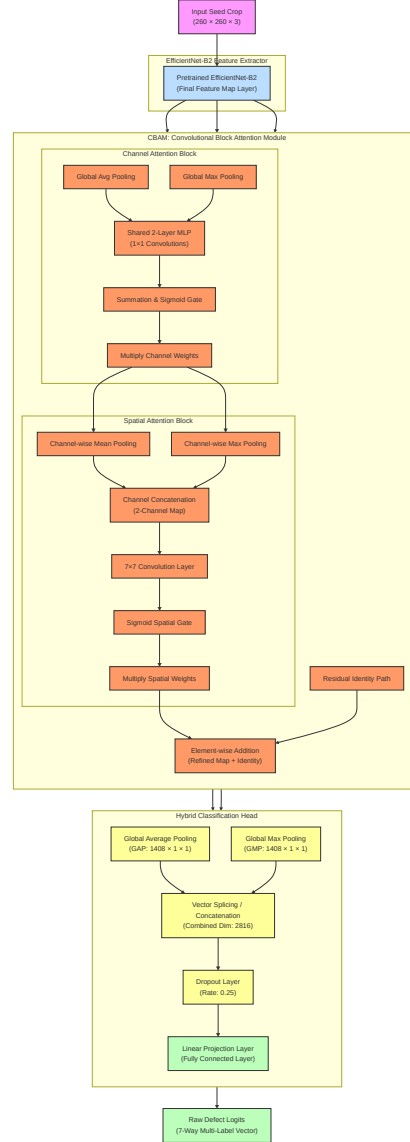
Figure 5.3: The EfficientNet-B2 defect classification architecture
