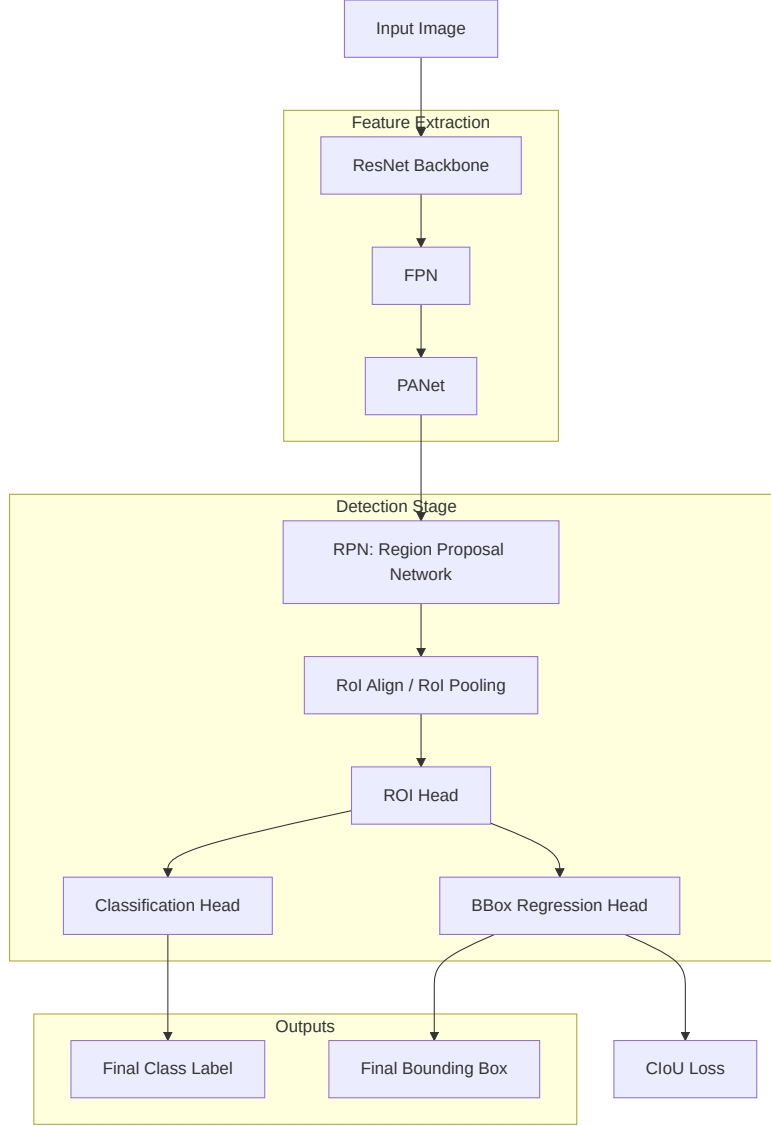
Figure 5.2: The Faster R-CNN detection architecture, showing the ResNet backbone, the FPN for multi-scale features, and the RPN and ROI head for detection and classification.
