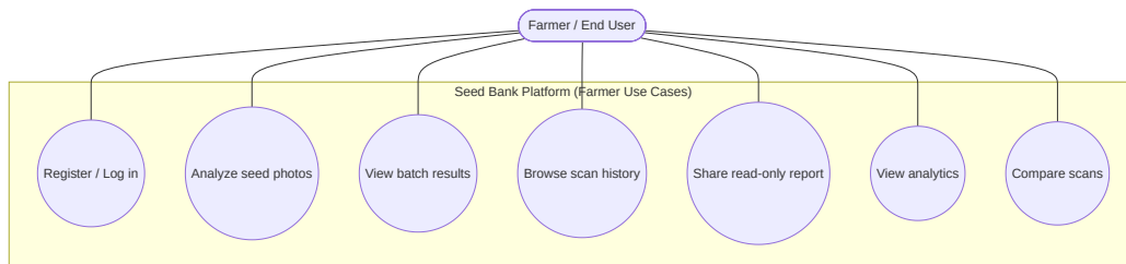
Figure 3.1: Use-case diagram: Farmer / End User.
