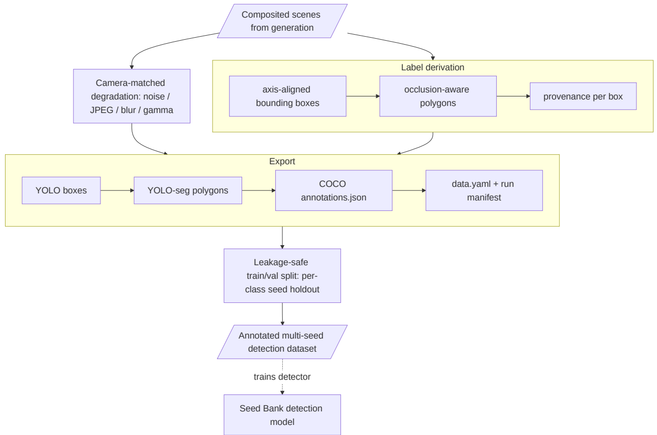
Figure 4.21: MultiSeedGen pipeline: derive per-seed labels from the composited scene, apply camera-matched degradation, and export leakage-safe detection and segmentation datasets.
