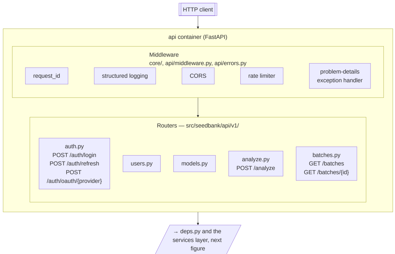
Figure 4.5: Backend request routing: HTTP client through middleware to the versioned routers.
