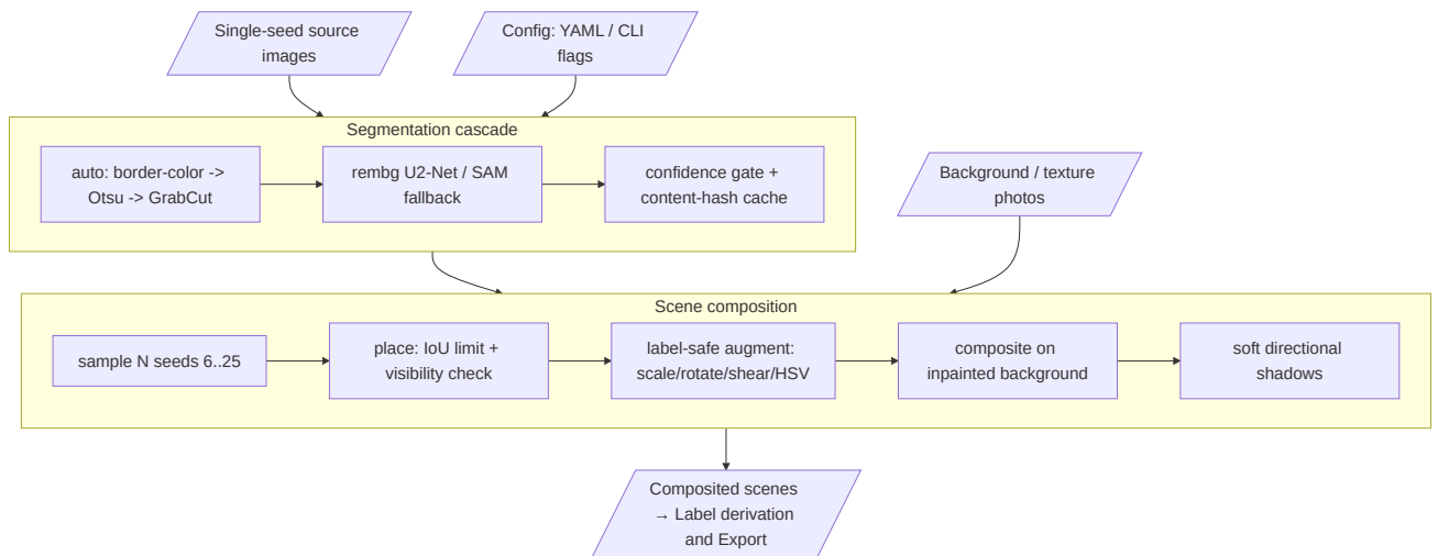
Figure 4.20: MultiSeedGen pipeline: segment single seeds and composite many onto varied backgrounds.
