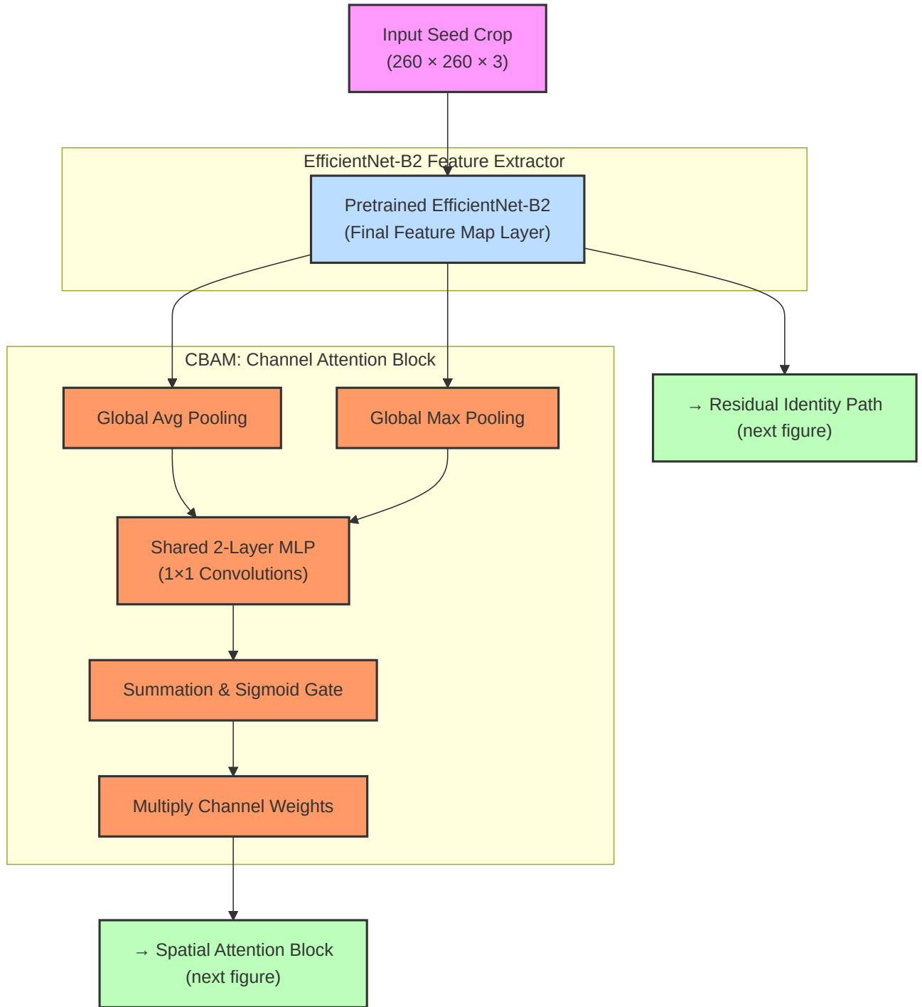
Figure 5.8: The EfficientNet-B2 backbone feeding the CBAM channel attention block.
