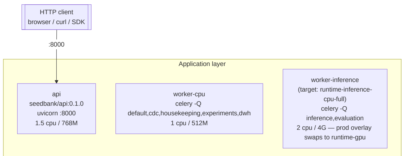
Figure 4.2: Container view: the application layer — the HTTP client, the API, and the two Celery workers.
