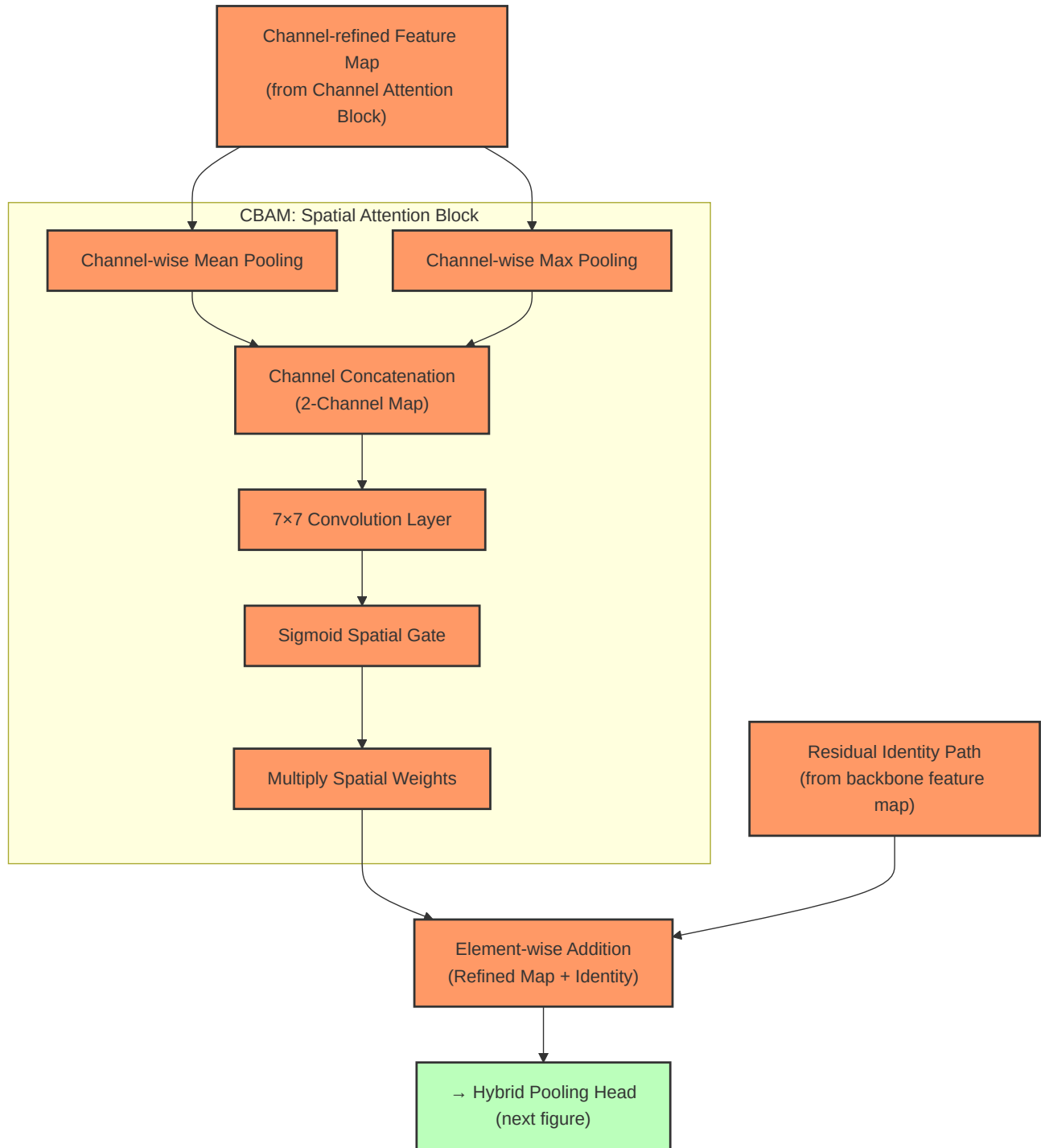
Figure 5.9: The CBAM spatial attention block, combining the channel-refined feature map with the residual identity path before the hybrid pooling head.
