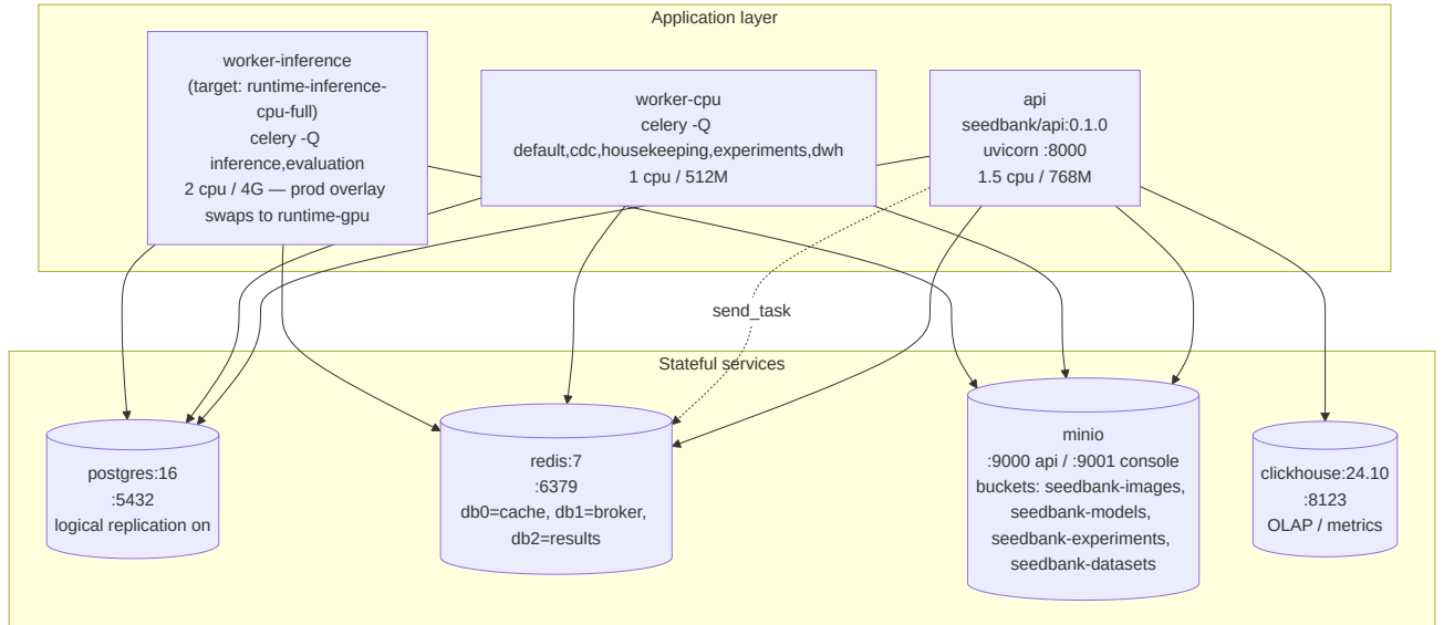
Figure 4.3: Container view: the application layer wired to its stateful datastores.
