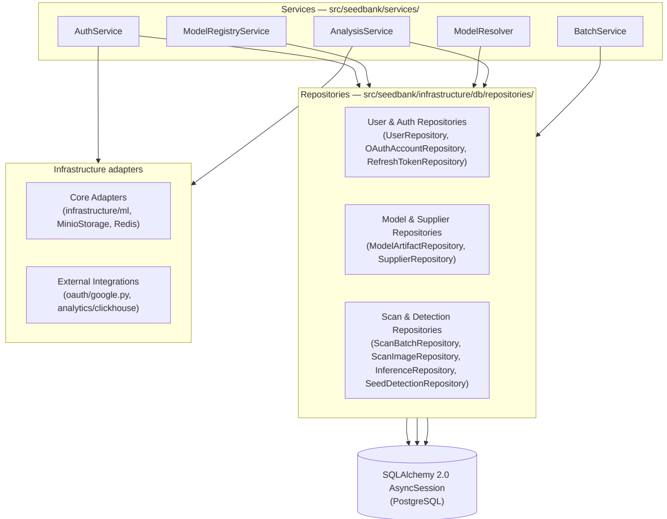
Figure 4.7: Backend data-access layer and repositories.
