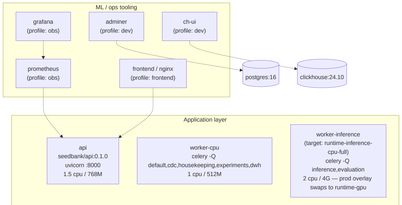
Figure 4.4: Container view: the application layer alongside the opt-in dev/obs/frontend tooling.
