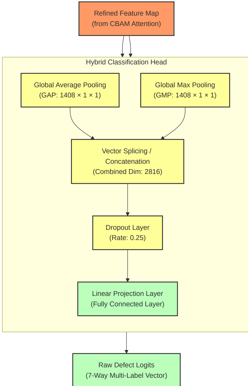
Figure 5.10: The hybrid pooling classification head, combining global average and max pooling on the CBAM-refined feature map before dropout and a final linear projection to defect logits.
