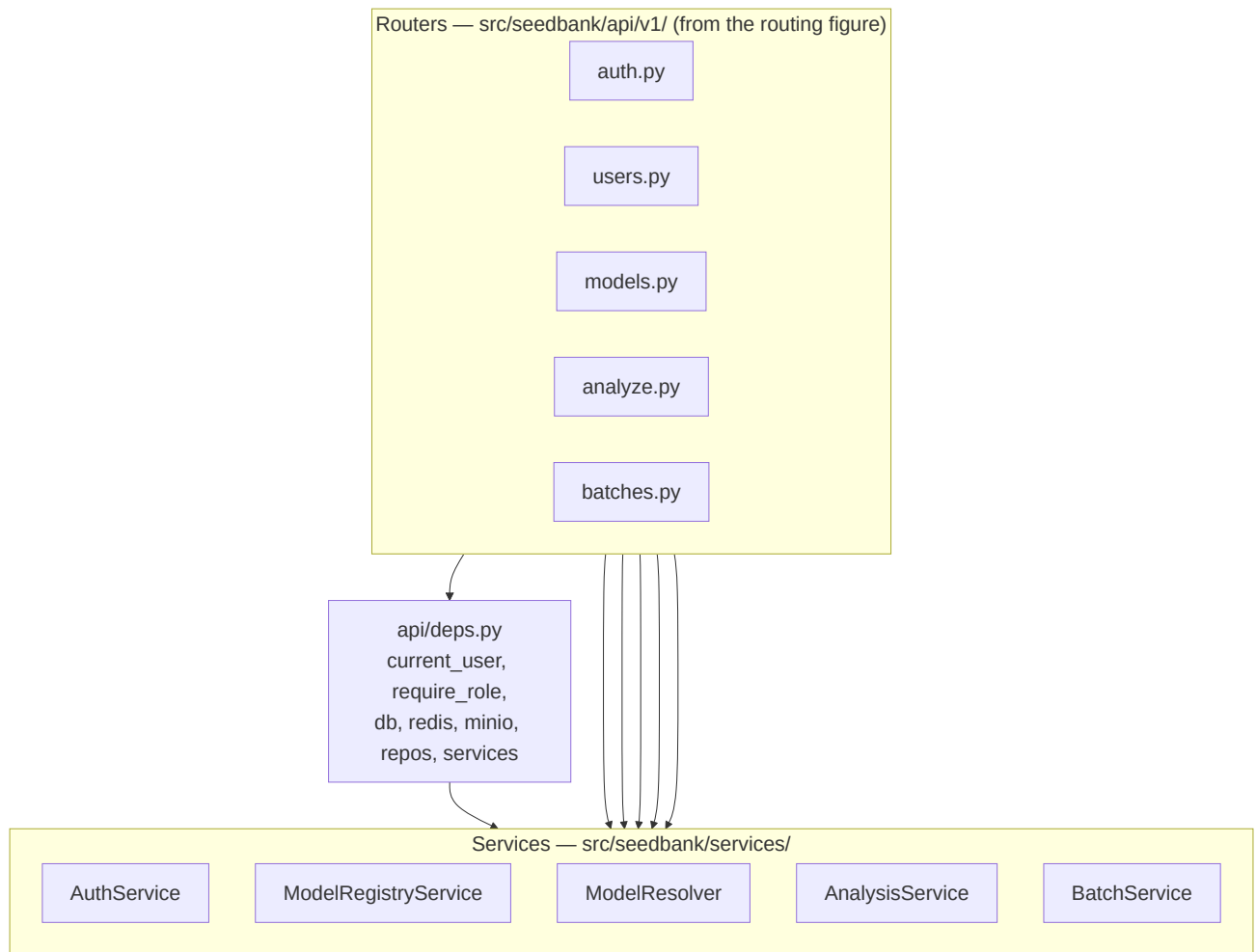
Figure 4.6: Backend request routing: routers through deps.py to the services layer.
