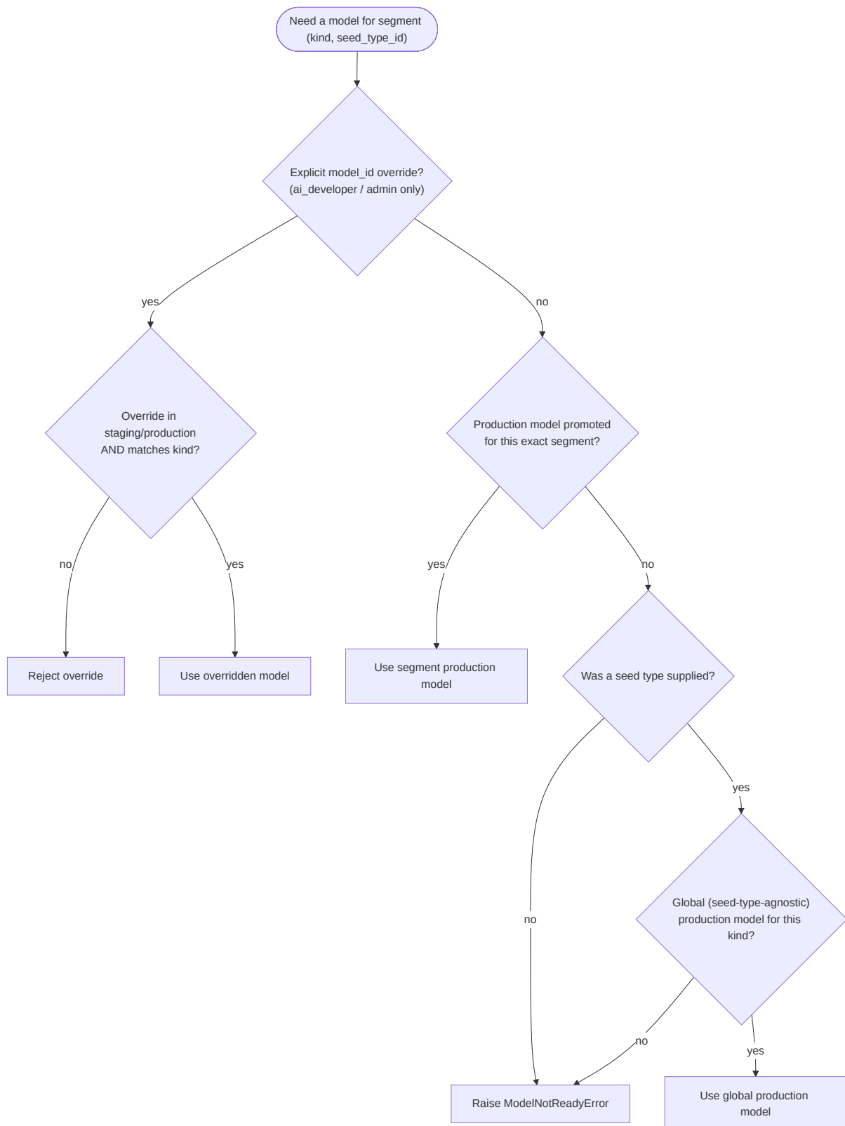
Figure 5.11: Model resolution: the resolver selects the model promoted to production for a segment, falls back to the global production model when only that is available, or reports that no model is ready.
