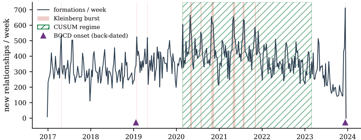
Global edge-formation series with three burst detectors
