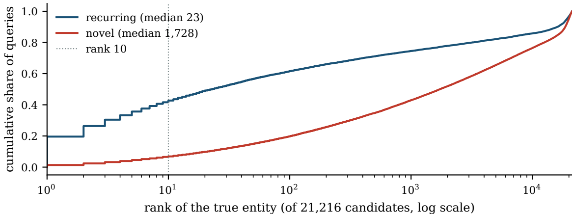
Where the truth ranks: recurring vs novel test edges (RE-GCN)
