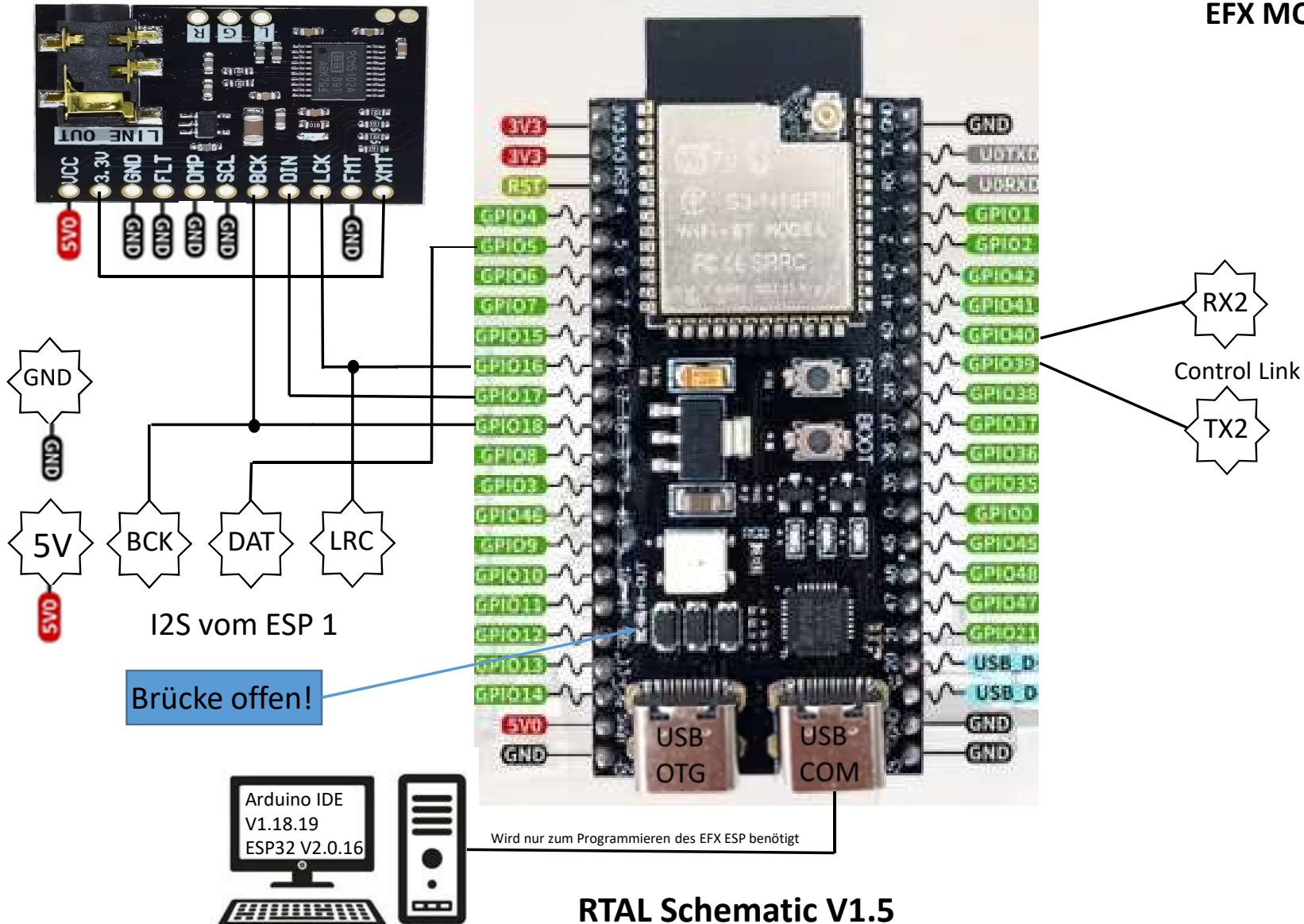
I2S DAC PCM 5102A
