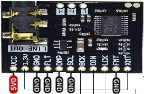
I2S DAC PCM 5102A
