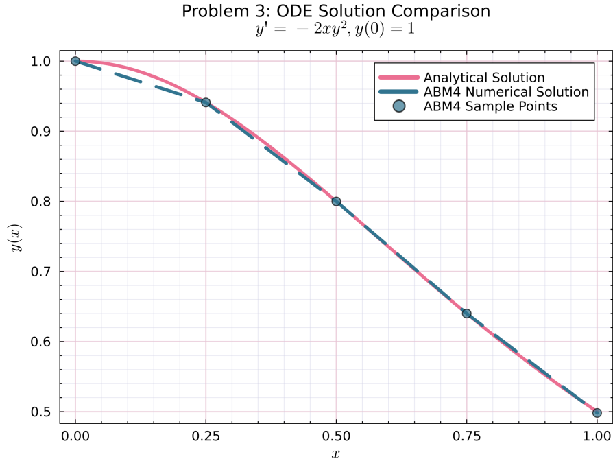
Figure 2: Comparison of ABM4 numerical solution (dashed blue line) with analytical solution (solid pink line). The markers indicate the discrete ABM4 sample points at x = 0, 0.25, 0.5, 0.75, 1.0 .
