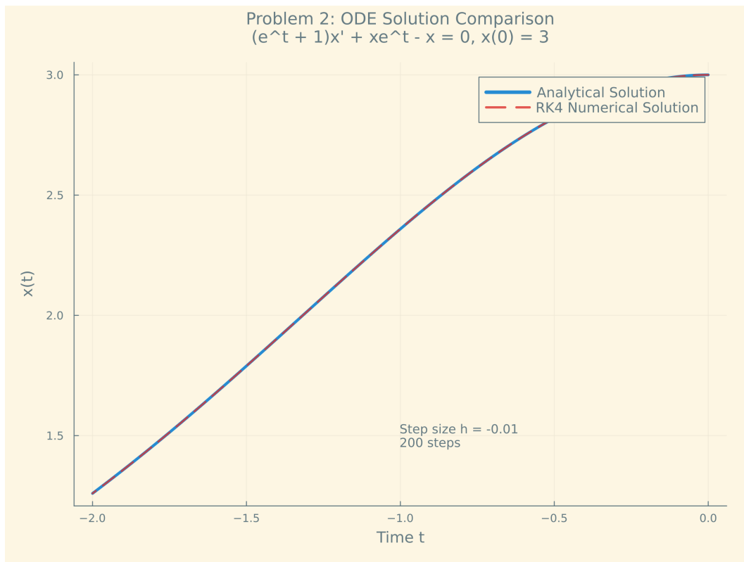
Figure 1: Comparison of RK4 numerical solution (red dashed) with analytical solution (blue solid) for the ODE (e^t + 1)x' + xe^t - x = 0 with x(0) = 3 . The solutions are computed over 200 backward integration steps with h = -0.01 .
