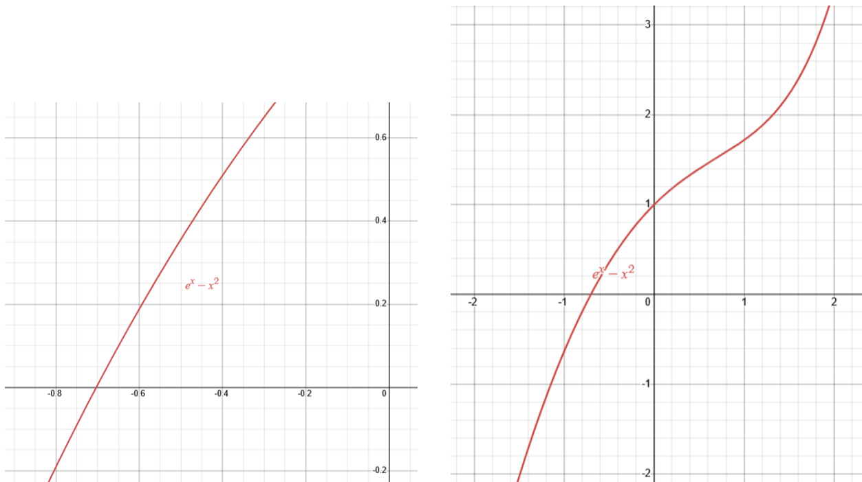
Figure 6: Graphs of e^x - x^2 : We can see from the zoomed in graph on the left that there is a single root in [-0.8, -0.6] . The zoomed out graph on the right shows that the function is monotonically increasing and has no other zeros.
