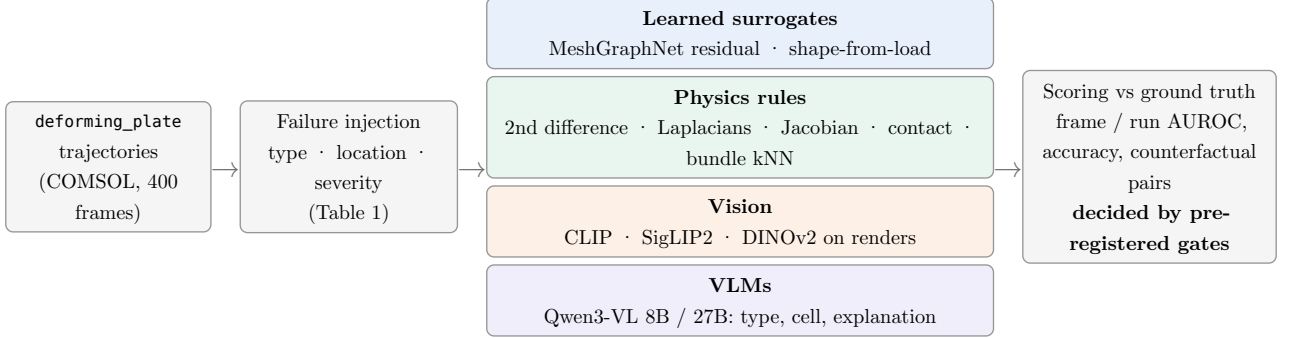
Figure 2: Study pipeline. Every detector family scores the same corrupted runs against the same injected ground truth; each comparison’s decision rule was committed before its data were scored.
