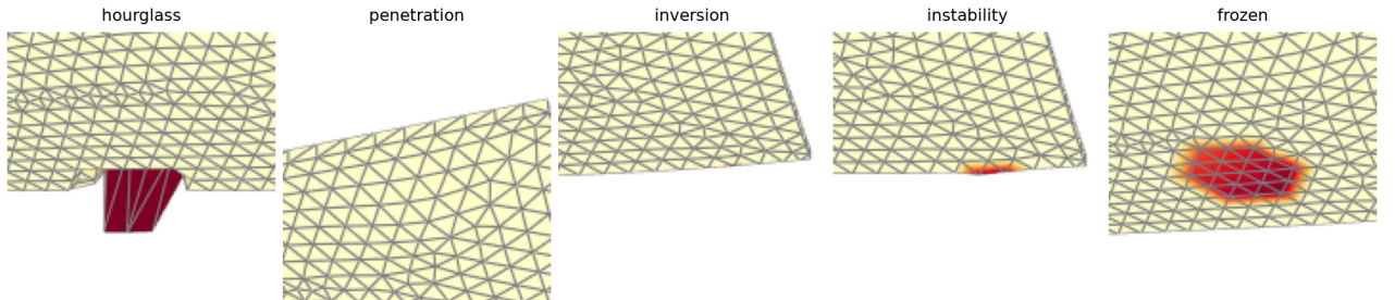
Figure 1: The five local failures at severity 3 (validation simulation 20), cropped around the injected region; the plate is coloured by deviation from the clean trajectory. Penetration and inversion occur on the underside at the actuator contact and are barely visible from the fixed camera used for all vision detectors.
