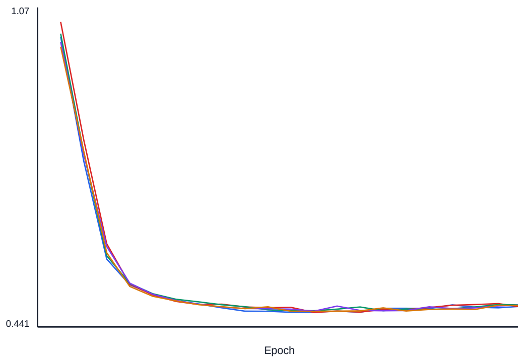
F-FNO
