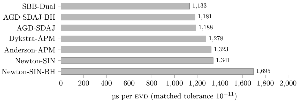
Figure 1: Median wall-clock time per EVD at n = 100 , all seven variants timed in one session. The spread is a factor of 1.50 and works against Newton, whose EVDs are accompanied by Krylov solves that the EVD count does not record. Anderson-APM’s EVDs cost 1.17 times SBB-Dual’s, the difference being its least-squares update of O(mn^2) work per EVD.
