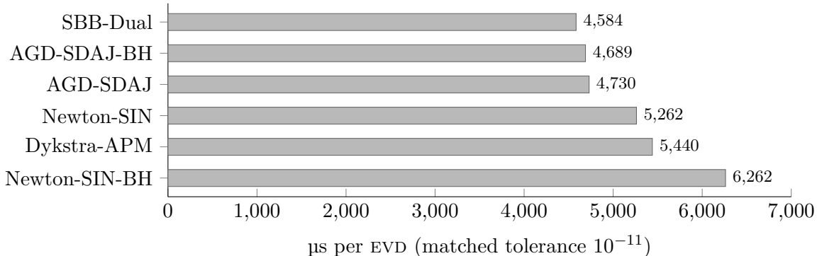
Figure 1: Median wall-clock time per EVD. The spread is a factor of 1.37 and works against Newton, whose EVDs are accompanied by Krylov solves that the EVD count does not record. Anderson-APM was added after these timing runs and is not shown; its extra work per EVD is a least-squares update of O(mn^2) .
